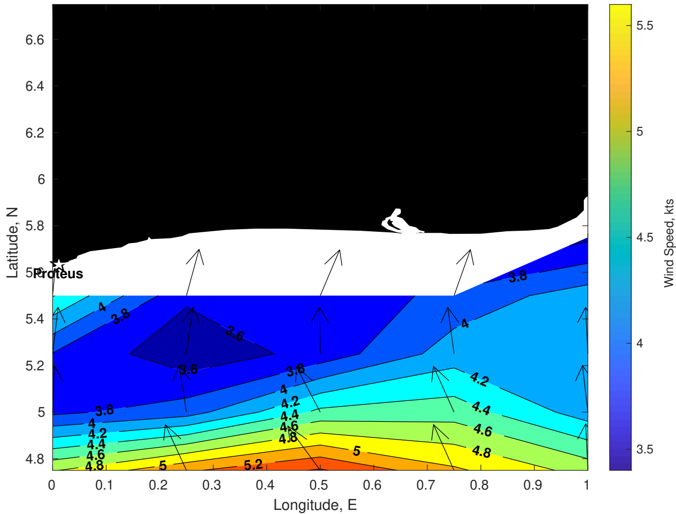
Winds (kts) for Proteus at 10-Nov-2025 09:00:00
