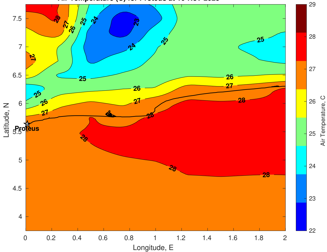
Air Temperature (C) for Proteus at 10-Nov-2025
