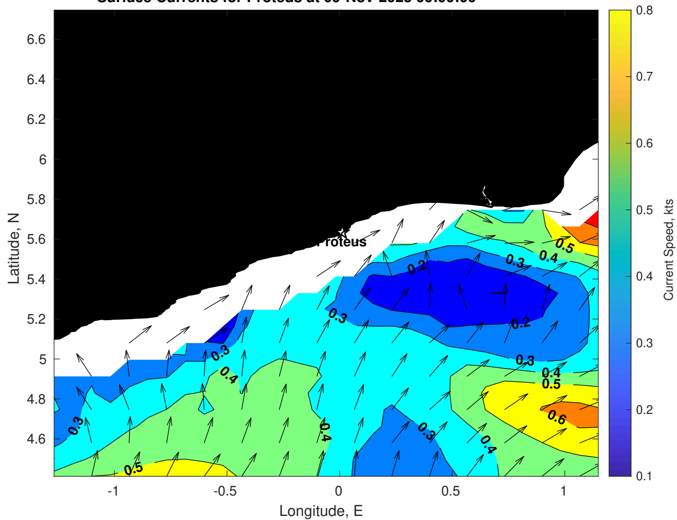
Surface Currents for Proteus at 09-Nov-2025 00:00:00
