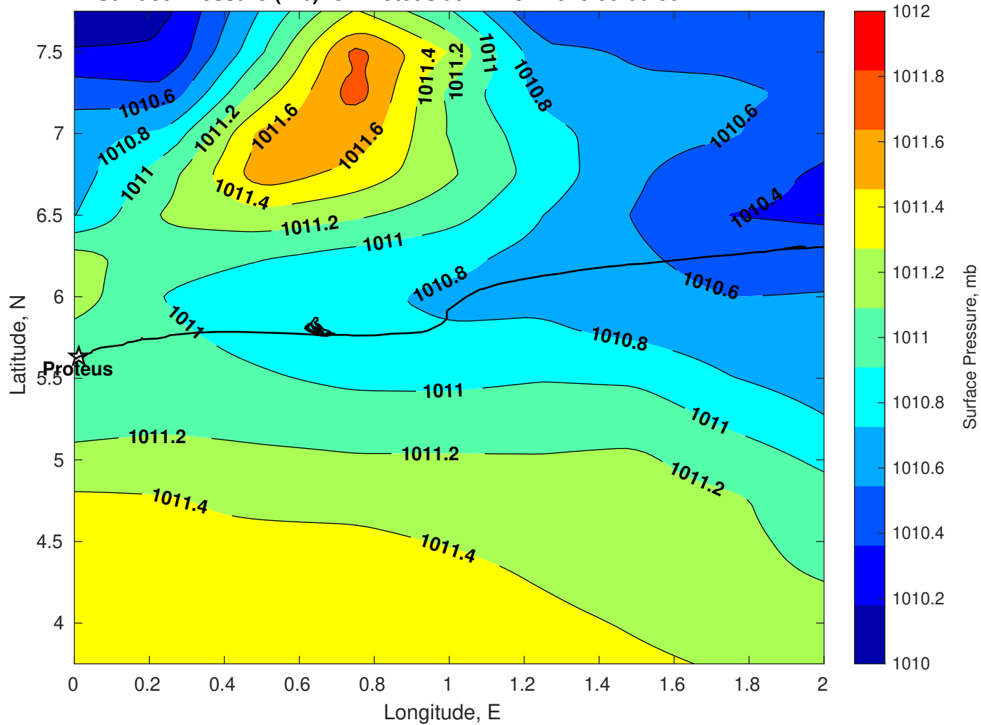
Surface Pressure (mb) for Proteus at 12-Nov-2025 00:00:00
