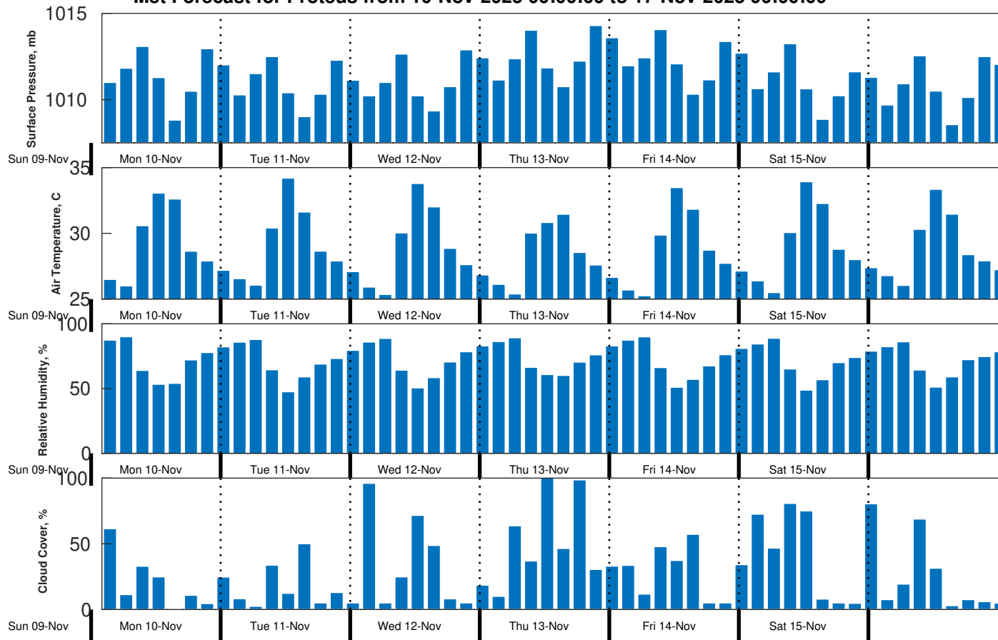
Met Forecast for Proteus from 10-Nov-2025 00:00:00 to 17-Nov-2025 00:00:00
