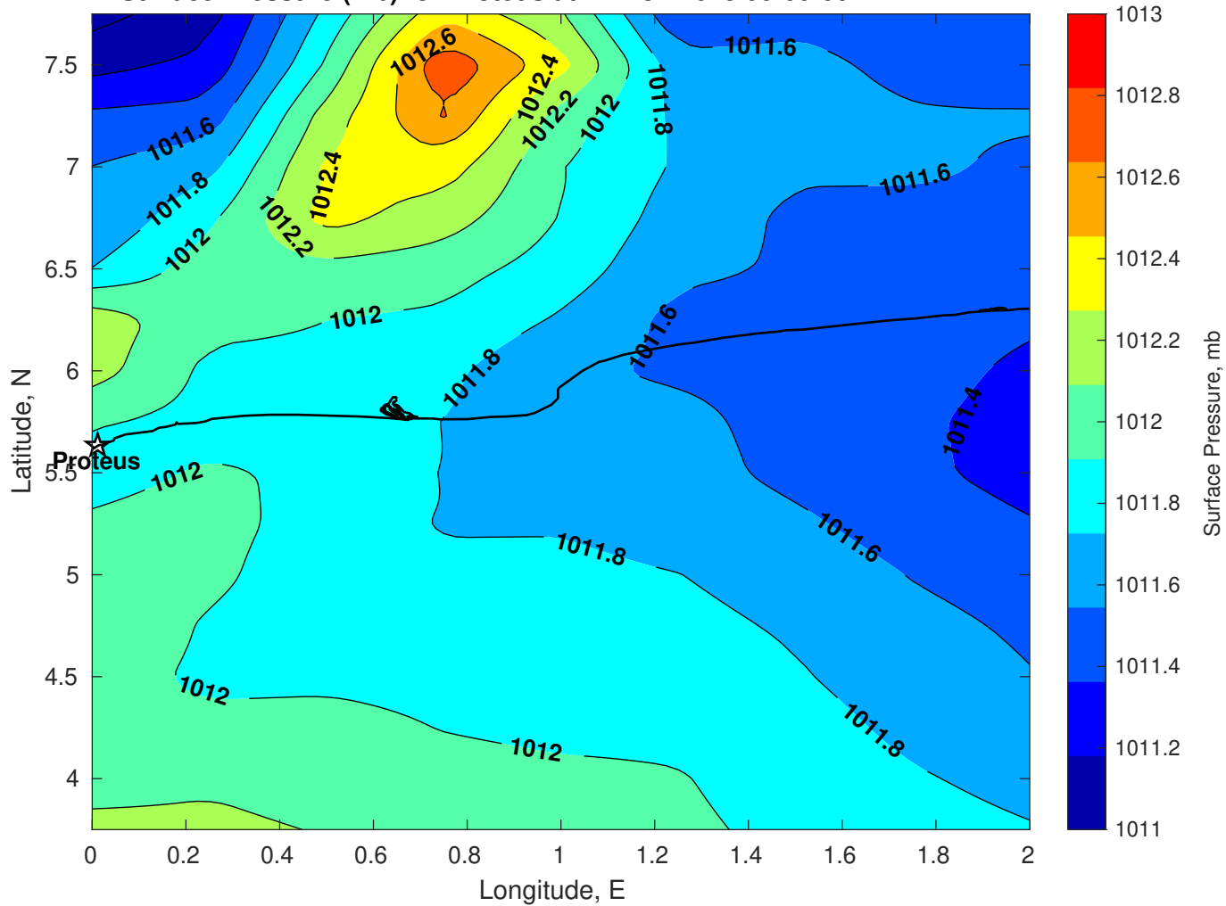
Surface Pressure (mb) for Proteus at 11-Nov-2025 00:00:00
