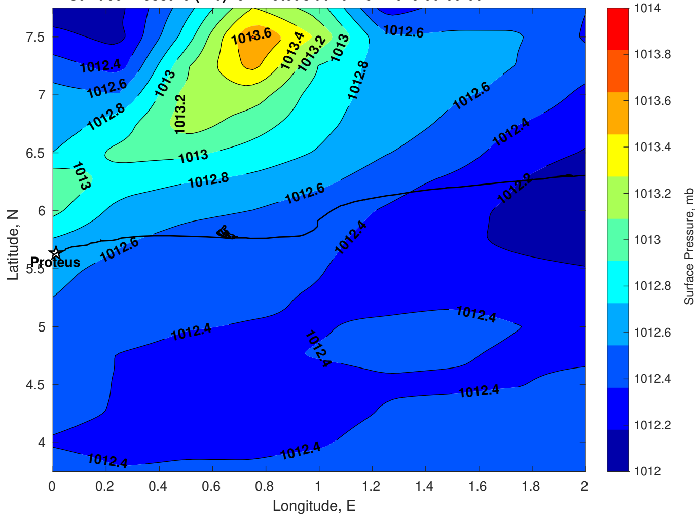
Surface Pressure (mb) for Proteus at 10-Nov-2025 00:00:00
