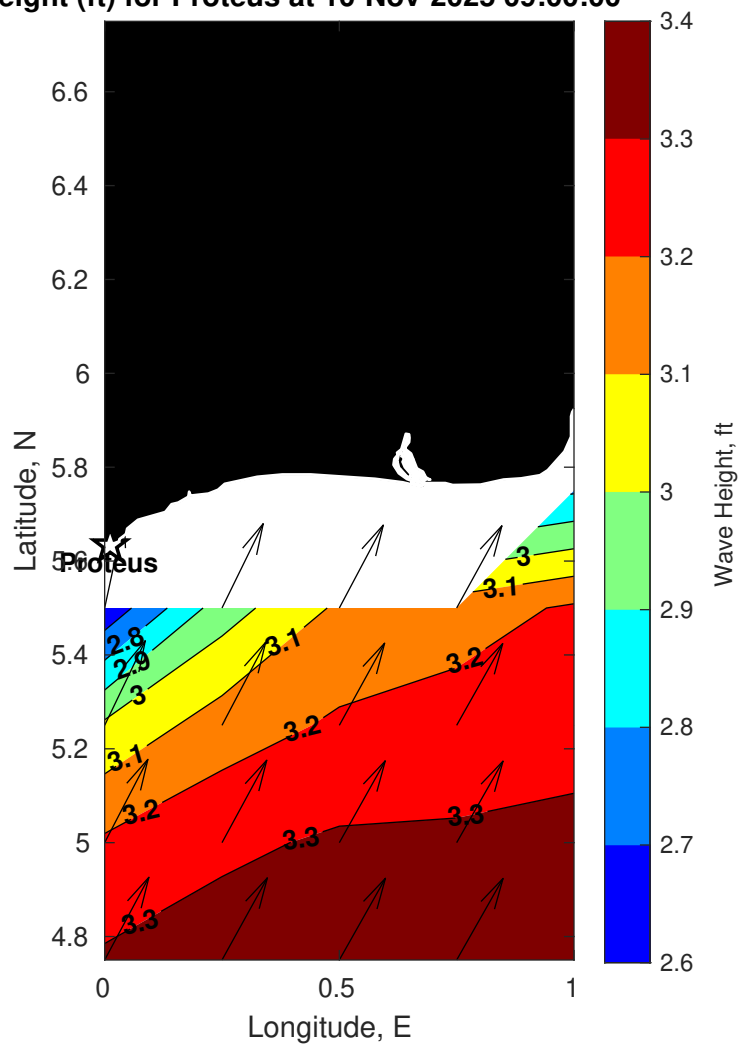
Wave Height (ft) for Proteus at 10-Nov-2025 09:00:00
