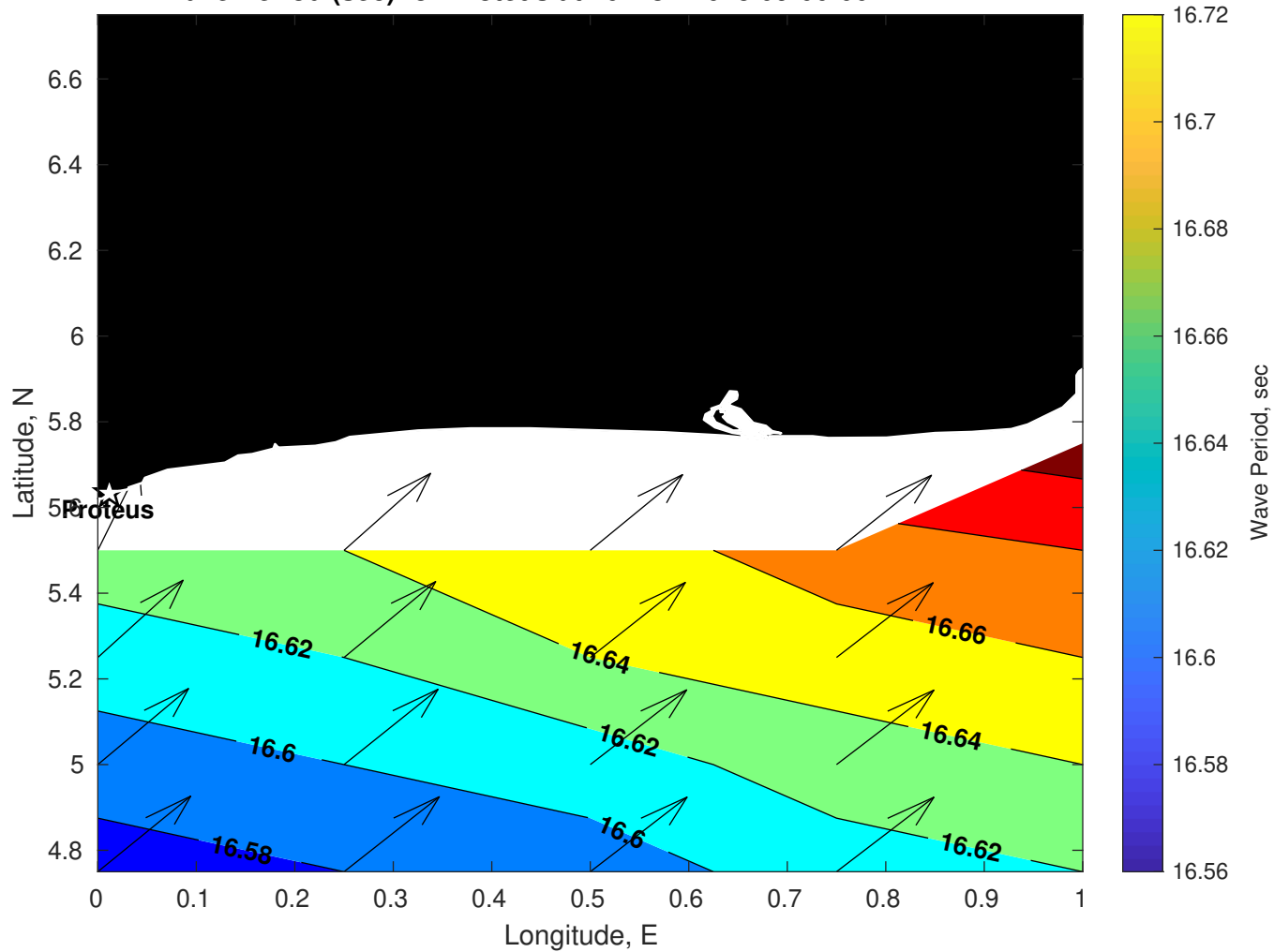
Wave Period (sec) for Proteus at 10-Nov-2025 09:00:00
