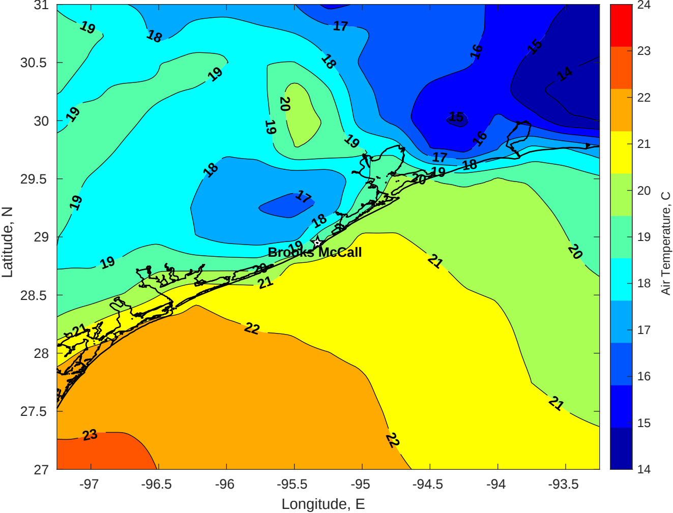
Air Temperature (C) for Brooks McCall at 11-Nov-2025
