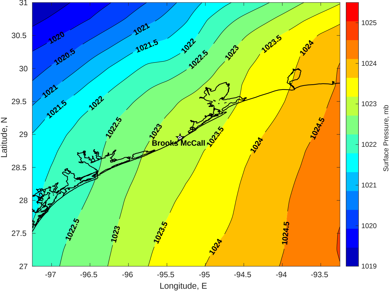
Surface Pressure (mb) for Brooks McCall at 12-Nov-2025 00:00:00
