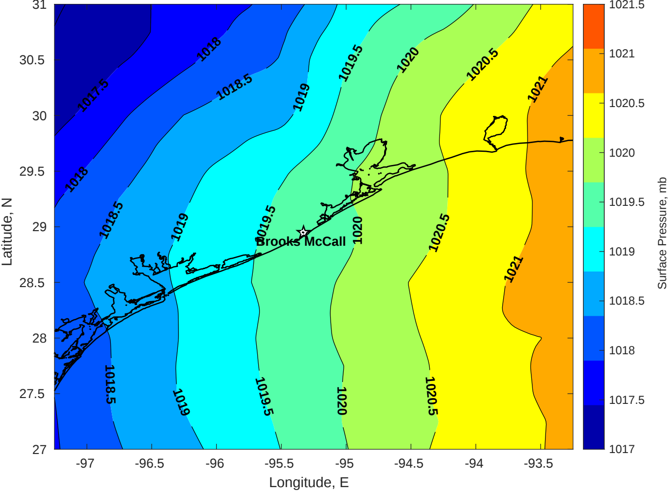
Surface Pressure (mb) for Brooks McCall at 13-Nov-2025 00:00:00
