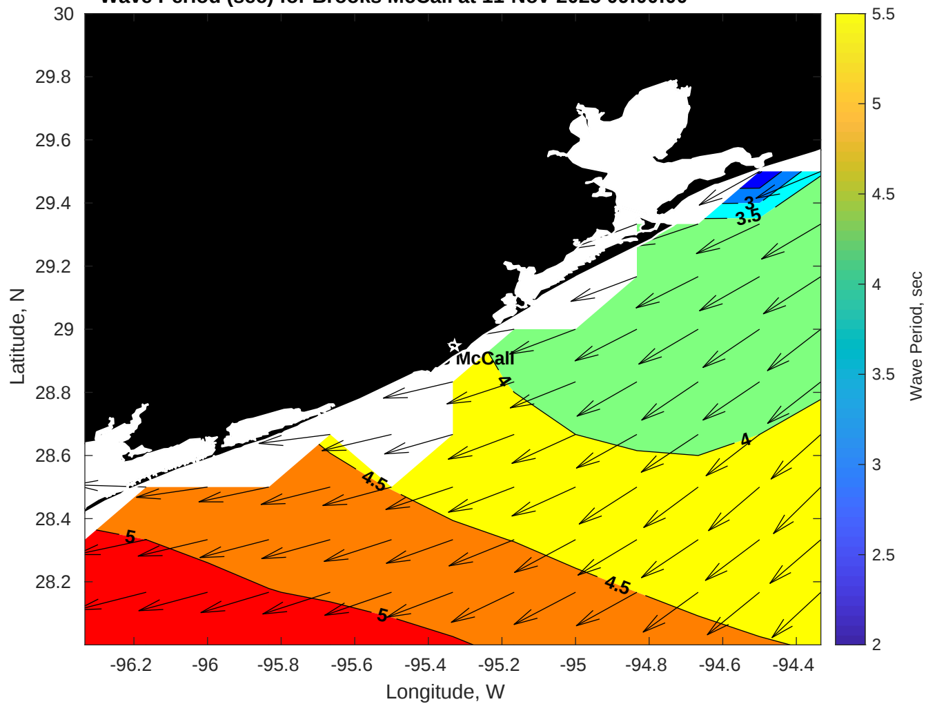
Wave Period (sec) for Brooks McCall at 11-Nov-2025 09:00:00
