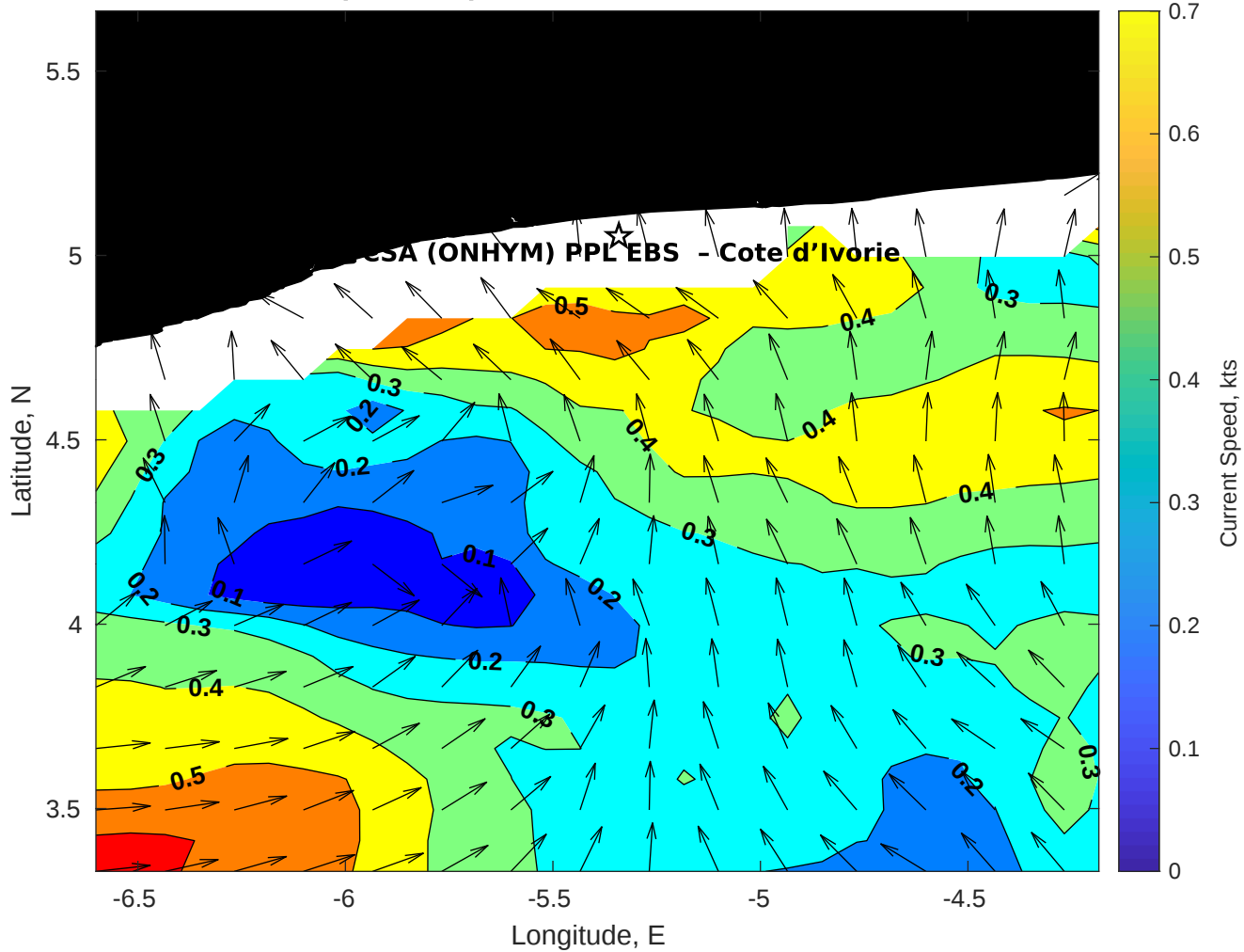
Surface Currents for CSA (ONHYM) PPL EBS - Cote d'Ivoire at 10-Nov-2025 00:00:00
