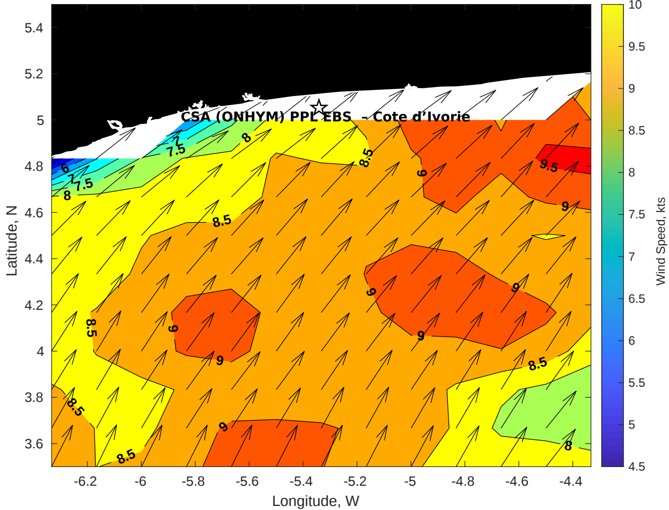
Winds (kts) for CSA (ONHYM) PPL EBS - Cote d'Ivoire at 11-Nov-2025 09:00:00
