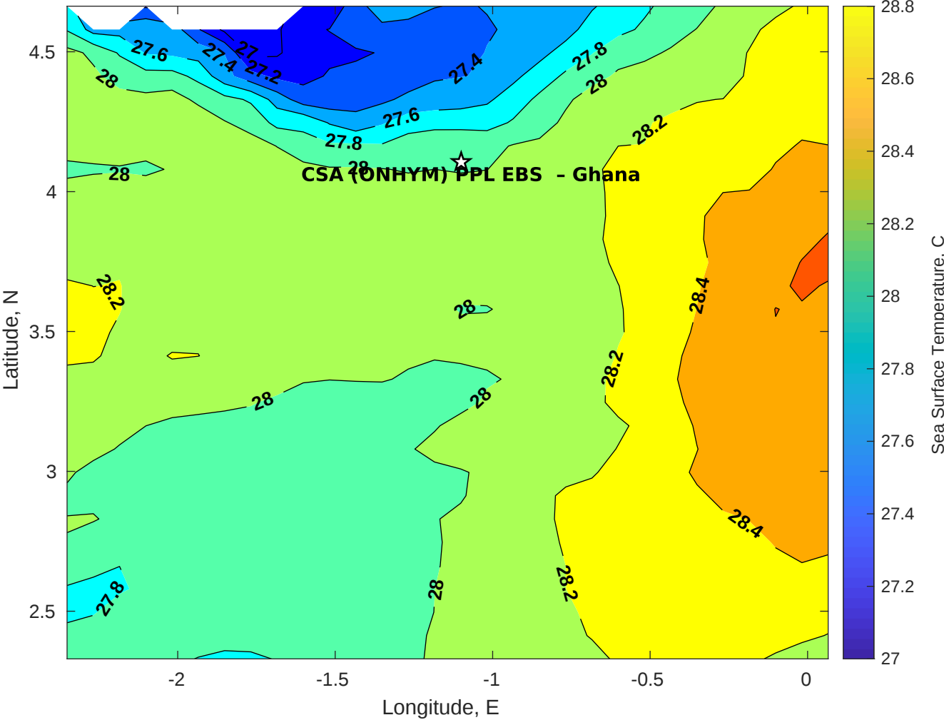
SST for CSA (ONHYM) PPL EBS - Ghana at 10-Nov-2025 00:00:00
