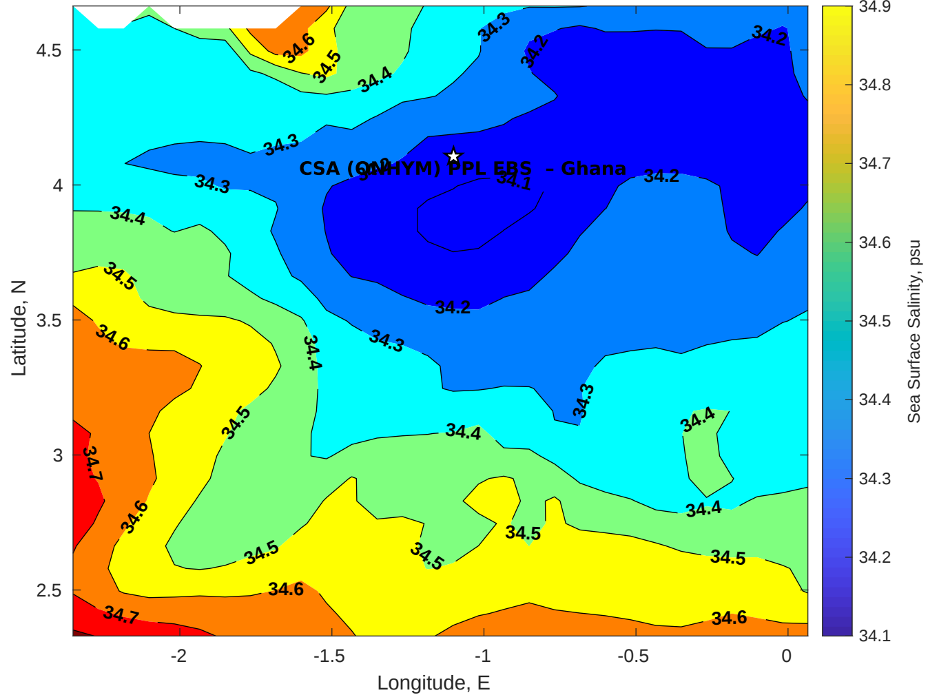
Surface Salinity for CSA (ONHYM) PPL EBS - Ghana at 10-Nov-2025 00:00:00
