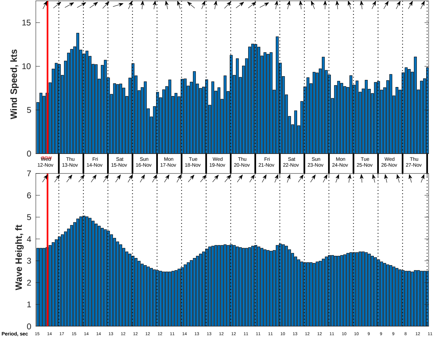
Wind & Wave Forecast for CSA (ONHYM) PPL EBS - Ghana from 11-Nov-2025 02:00:00 to 27-Nov-2025 02:00:00
