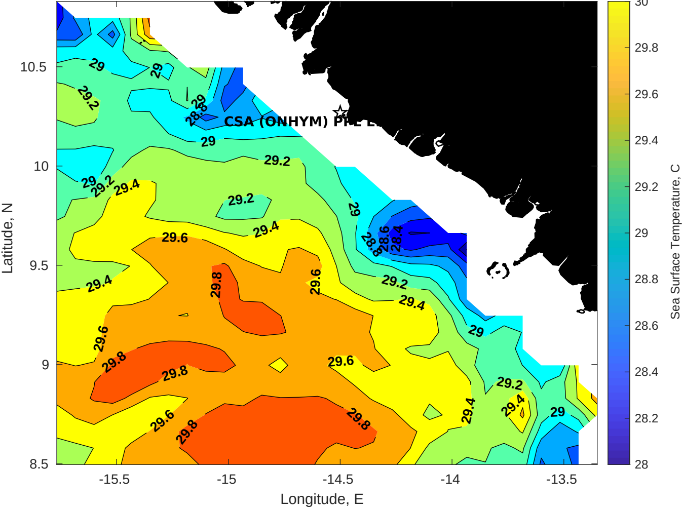
SST for CSA (ONHYM) PPL EBS - Guinea at 10-Nov-2025 00:00:00
