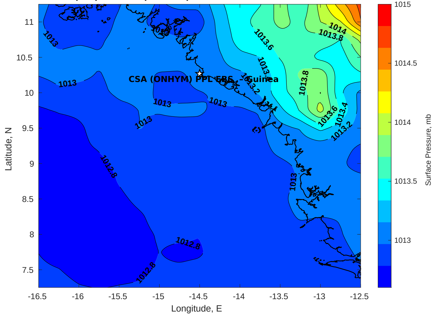
Surface Pressure (mb) for CSA (ONHYM) PPL EBS - Guinea at 12-Nov-2025 00:00:00
