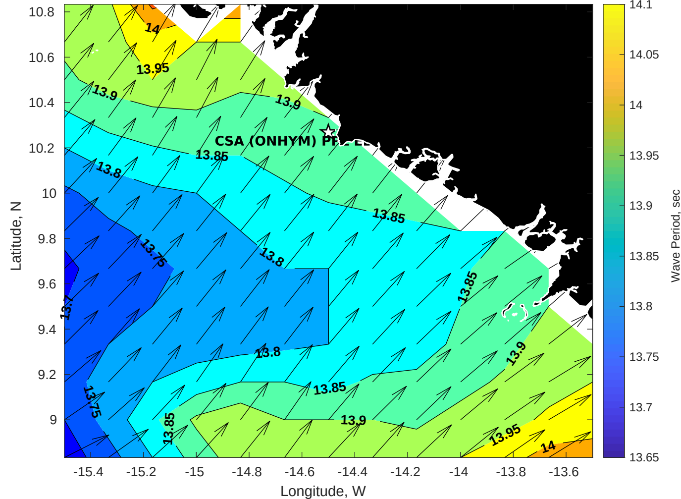
Wave Period (sec) for CSA (ONHYM) PPL EBS - Guinea at 11-Nov-2025 09:00:00
