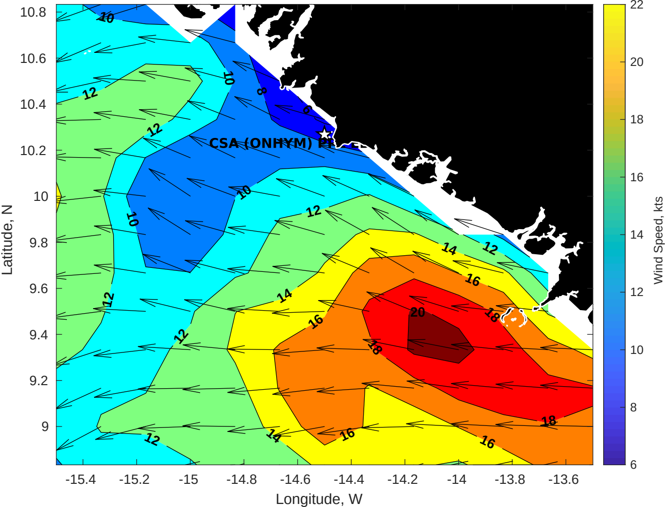
Winds (kts) for CSA (ONHYM) PPL EBS - Guinea at 11-Nov-2025 09:00:00
