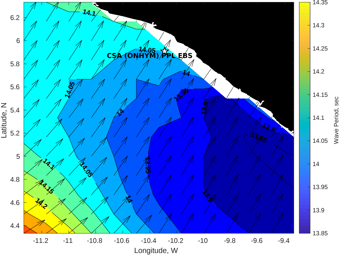
Wave Period (sec) for CSA (ONHYM) PPL EBS - Liberia at 11-Nov-2025 09:00:00
