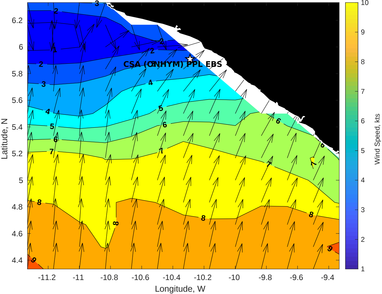
Winds (kts) for CSA (ONHYM) PPL EBS - Liberia at 11-Nov-2025 09:00:00
