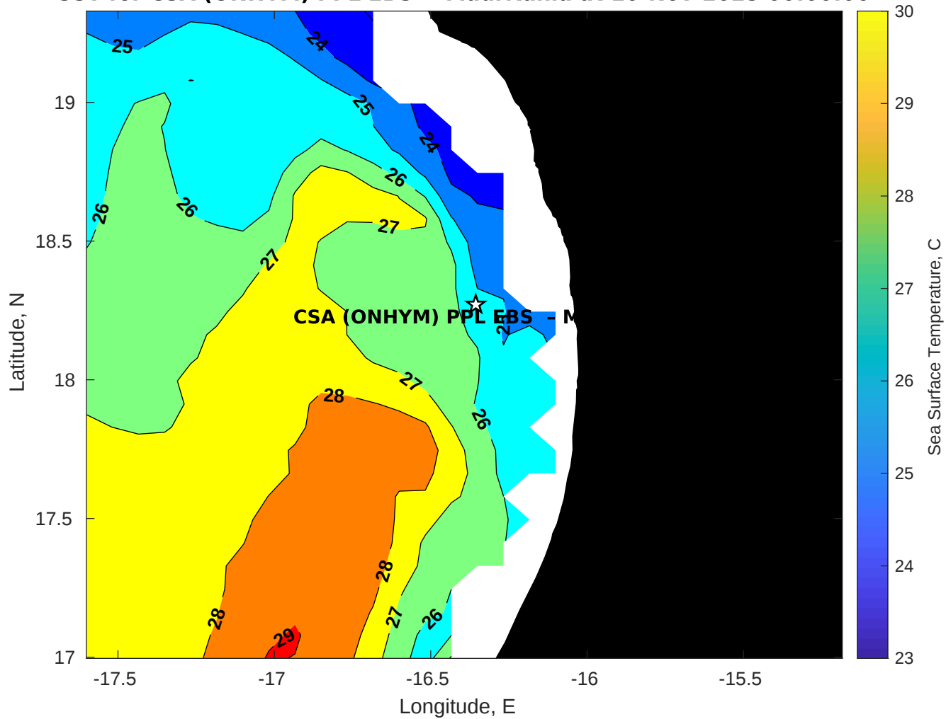
SST for CSA (ONHYM) PPL EBS - Mauritania at 10-Nov-2025 00:00:00
