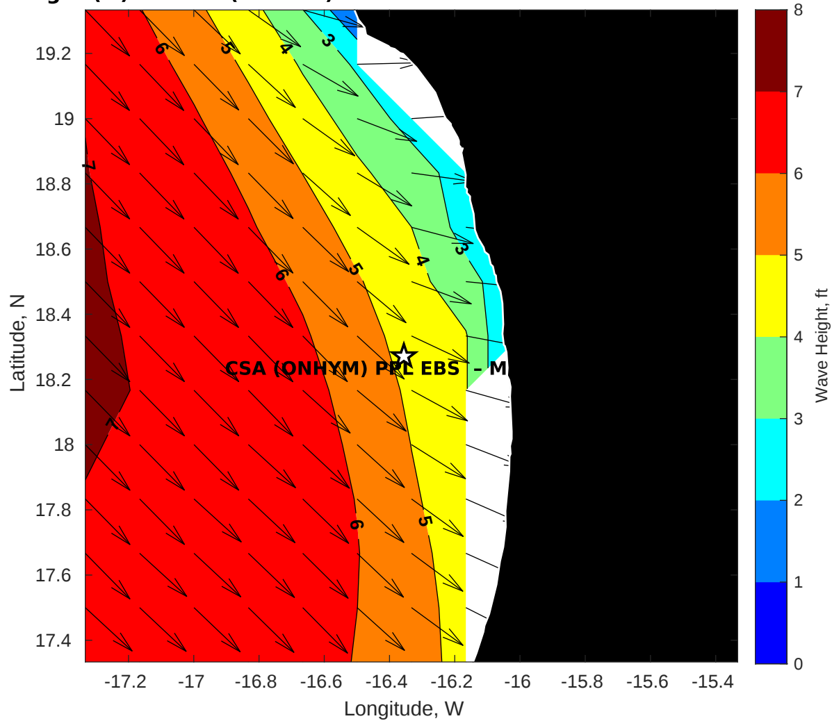
Wave Height (ft) for CSA (ONHYM) PPL EBS - Mauritania at 11-Nov-2025 09:00:00
