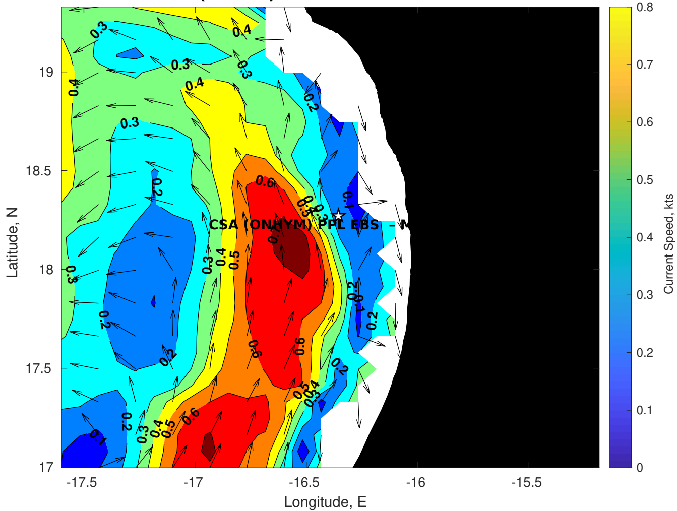
Surface Currents for CSA (ONHYM) PPL EBS - Mauritania at 10-Nov-2025 00:00:00
