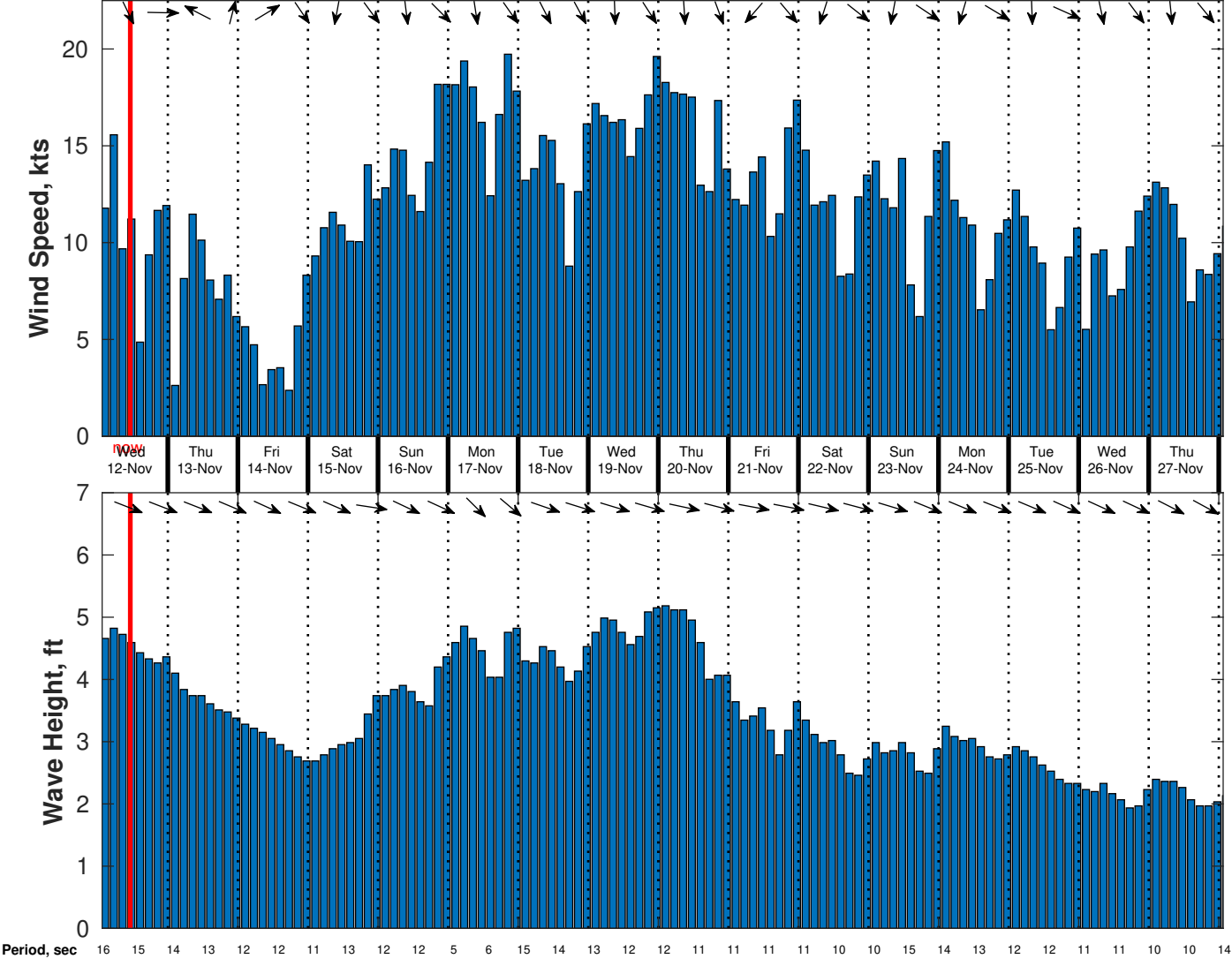
Wind & Wave Forecast for CSA (ONHYM) PPL EBS - Mauritania from 11-Nov-2025 01:00:00 to 27-Nov-2025 01:00:00
