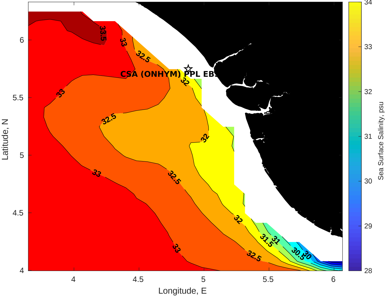
Surface Salinity for CSA (ONHYM) PPL EBS - Nigeria at 10-Nov-2025 00:00:00
