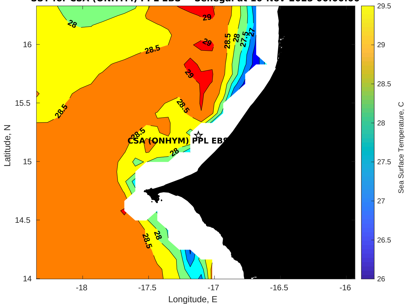
SST for CSA (ONHYM) PPL EBS - Senegal at 10-Nov-2025 00:00:00
