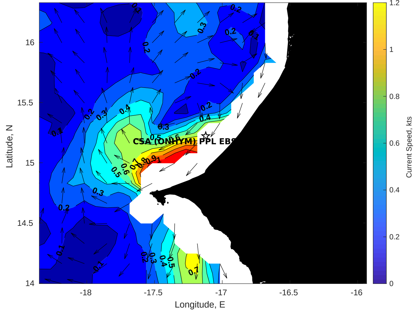
Surface Currents for CSA (ONHYM) PPL EBS - Senegal at 10-Nov-2025 00:00:00
