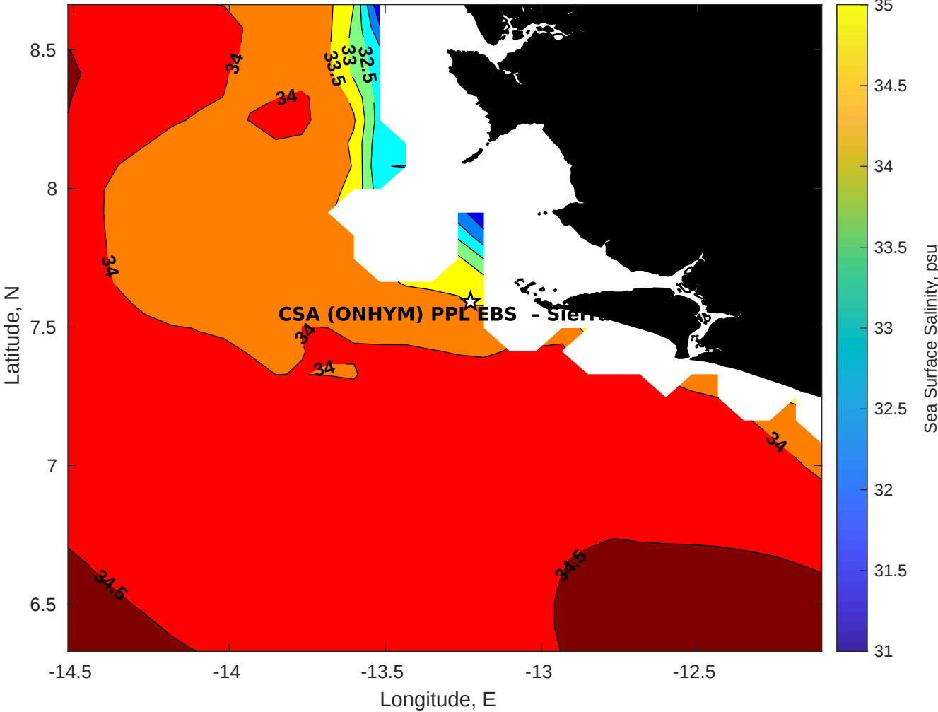
Surface Salinity for CSA (ONHYM) PPL EBS - Sierra Leone at 10-Nov-2025 00:00:00
