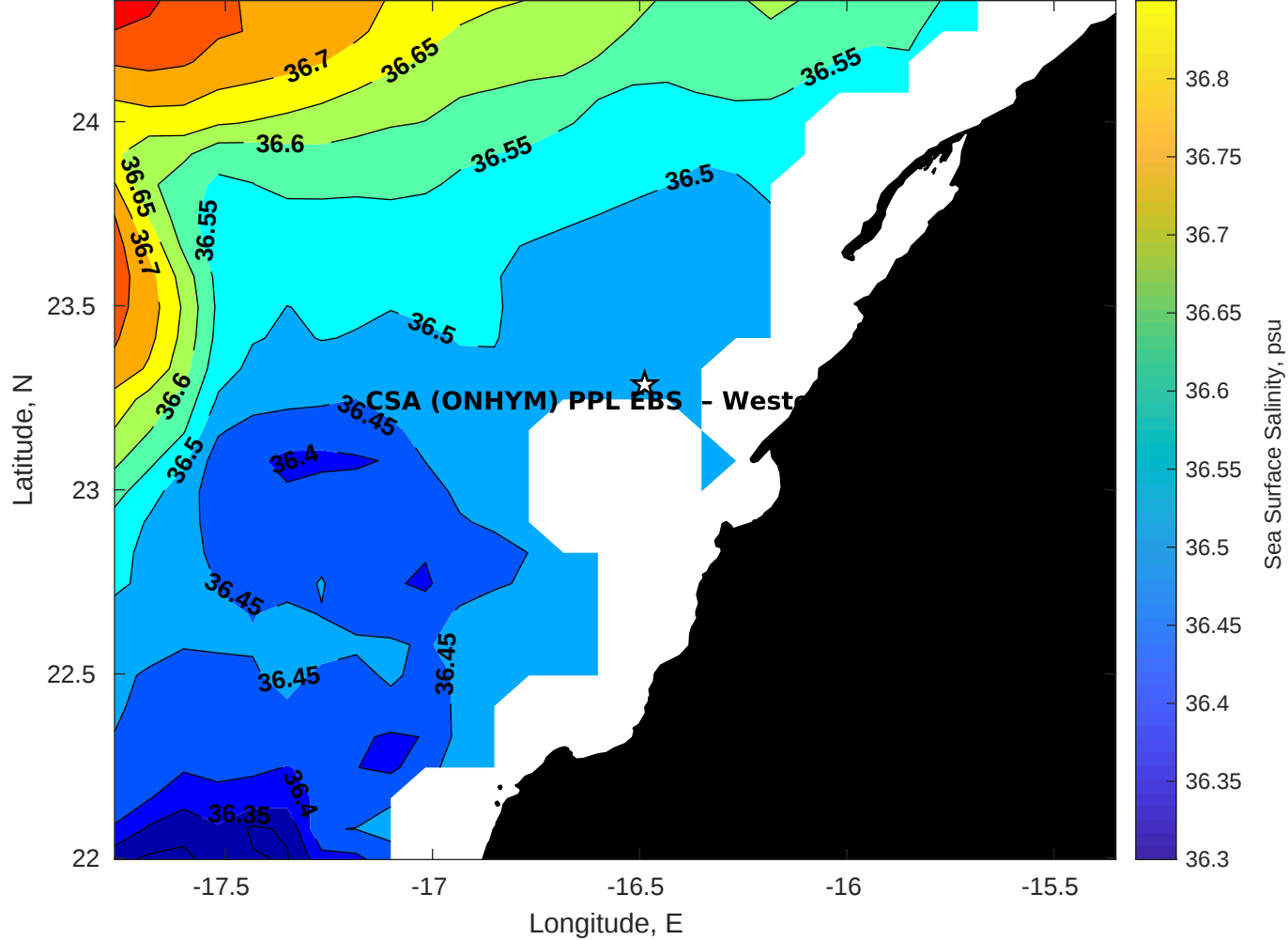
Surface Salinity for CSA (ONHYM) PPL EBS - Western Sahara at 10-Nov-2025 00:00:00
