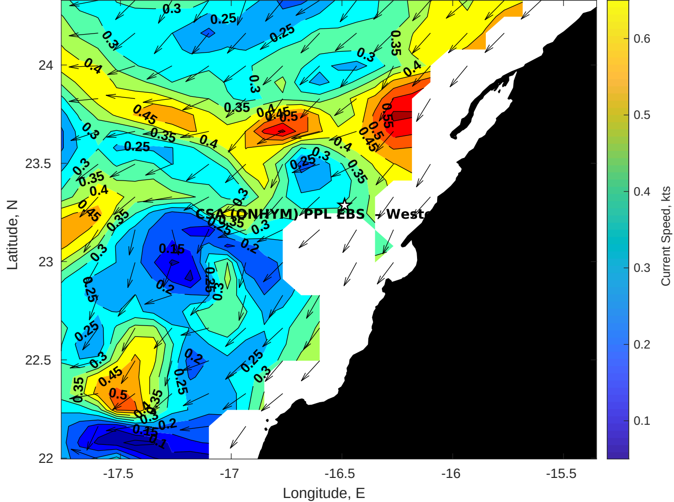
Surface Currents for CSA (ONHYM) PPL EBS - Western Sahara at 10-Nov-2025 00:00:00
