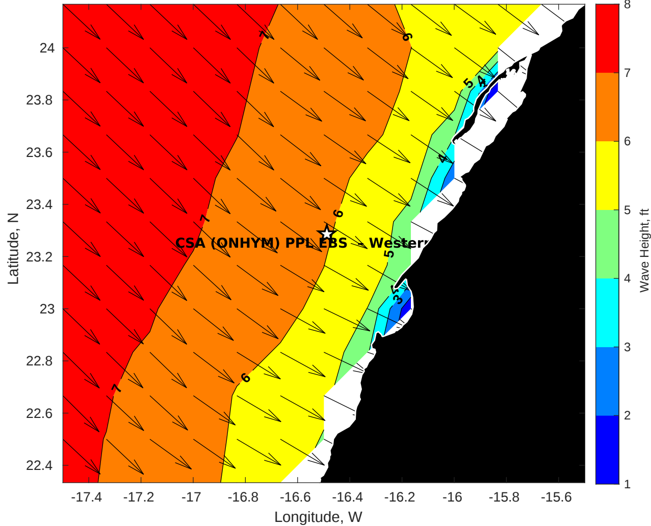
Wave Height (ft) for CSA (ONHYM) PPL EBS - Western Sahara at 11-Nov-2025 09:00:00
