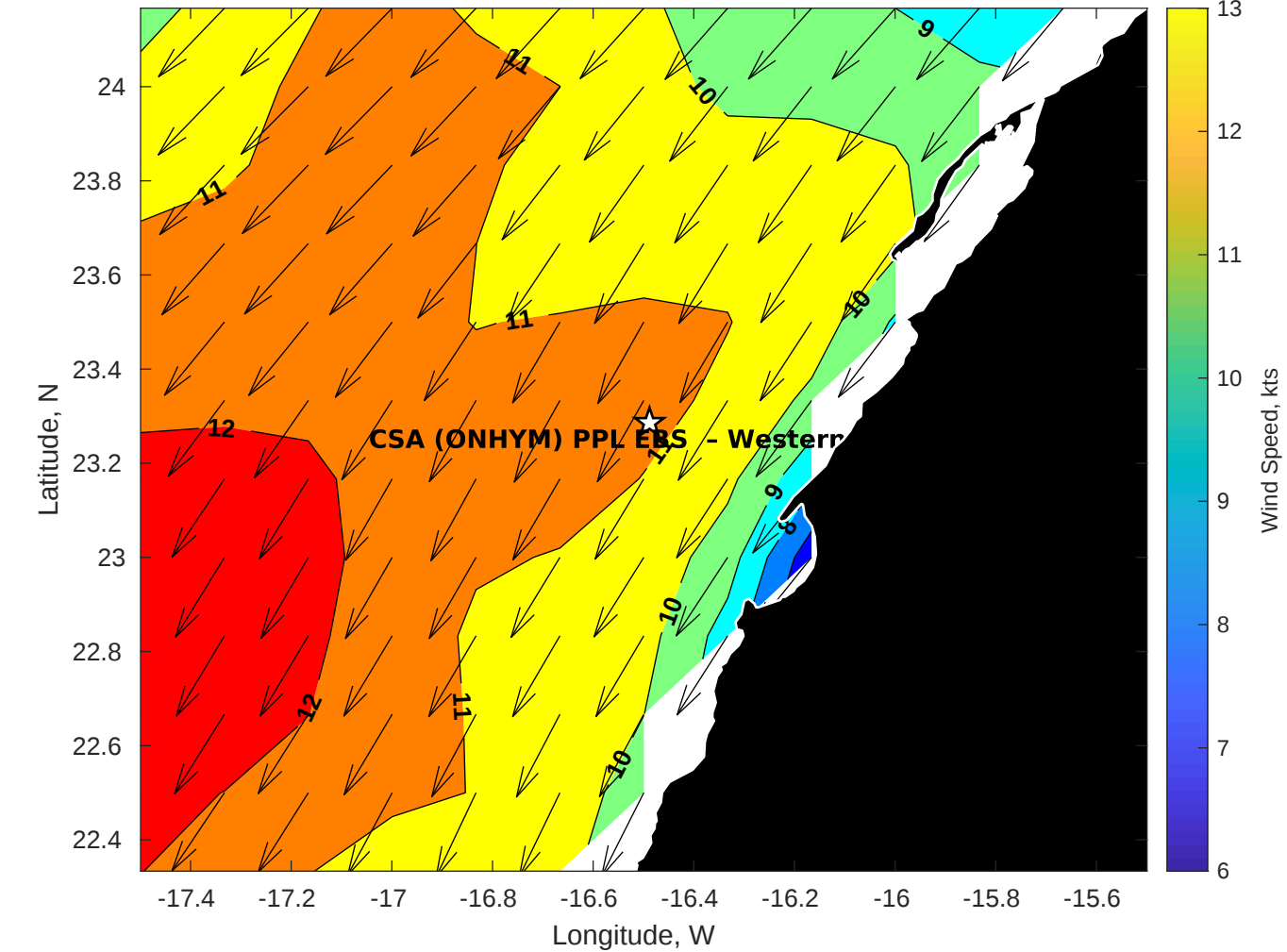
Winds (kts) for CSA (ONHYM) PPL EBS - Western Sahara at 11-Nov-2025 09:00:00
