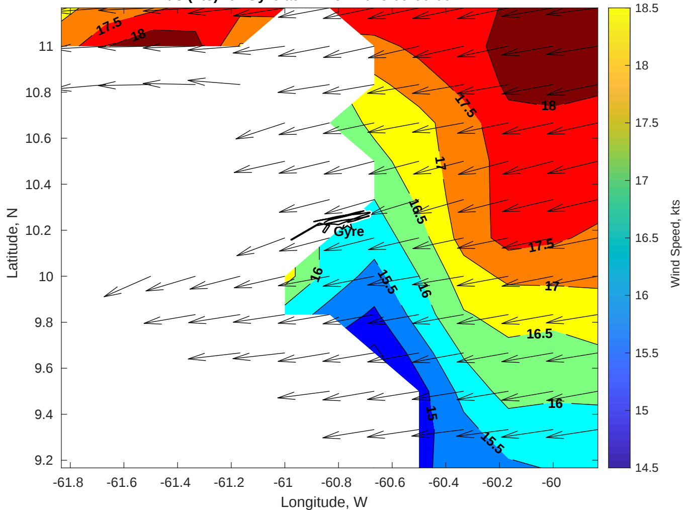
Winds (kts) for Gyre at 11-Nov-2025 09:00:00
