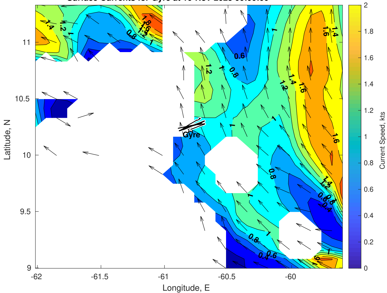
Surface Currents for Gyre at 10-Nov-2025 00:00:00
