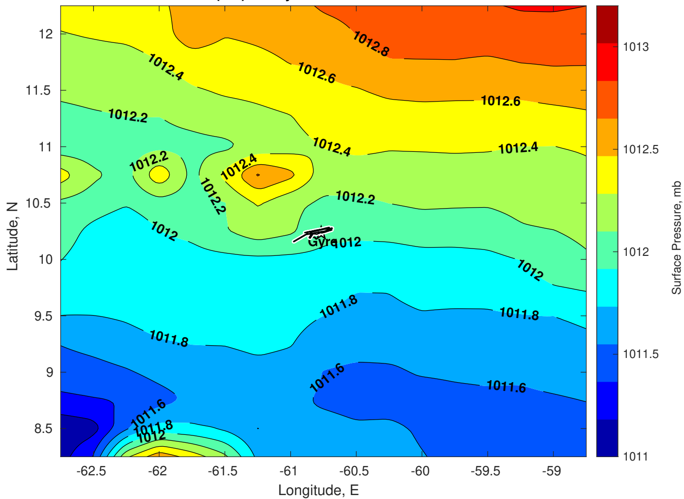
Surface Pressure (mb) for Gyre at 13-Nov-2025 00:00:00
