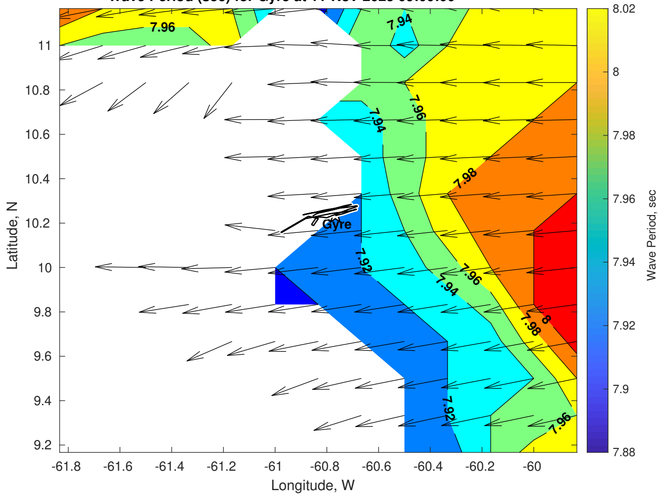
Wave Period (sec) for Gyre at 11-Nov-2025 09:00:00
