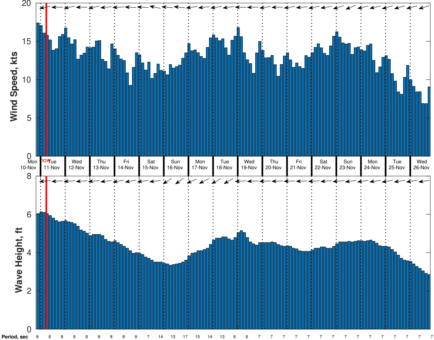
Wind & Wave Forecast for Gyre from 10-Nov-2025 20:00:00 to 26-Nov-2025 20:00:00
