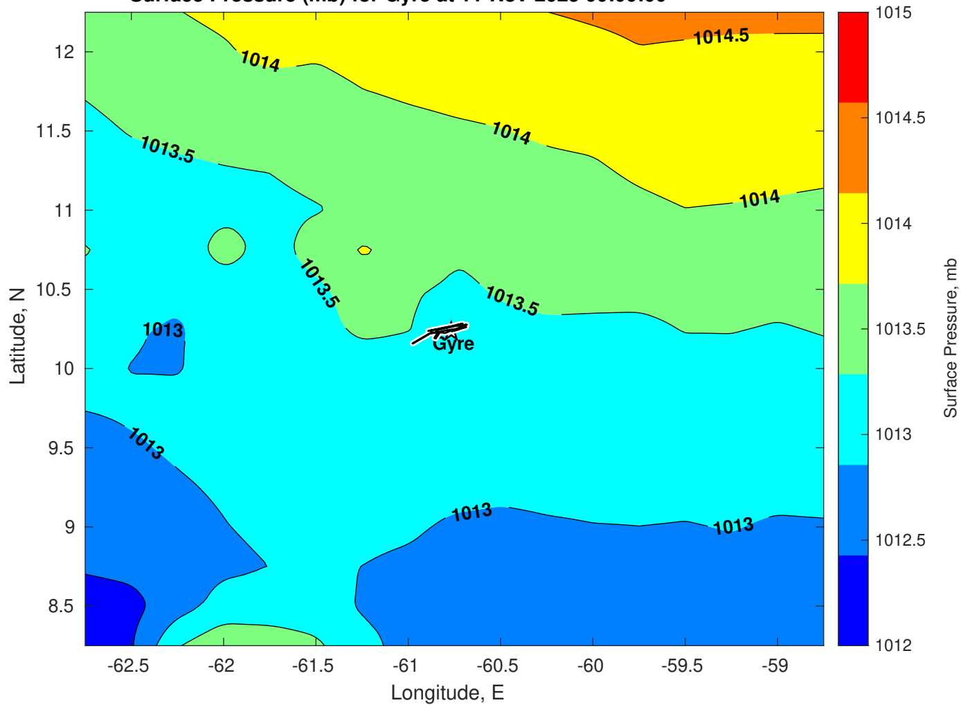
Surface Pressure (mb) for Gyre at 11-Nov-2025 00:00:00
