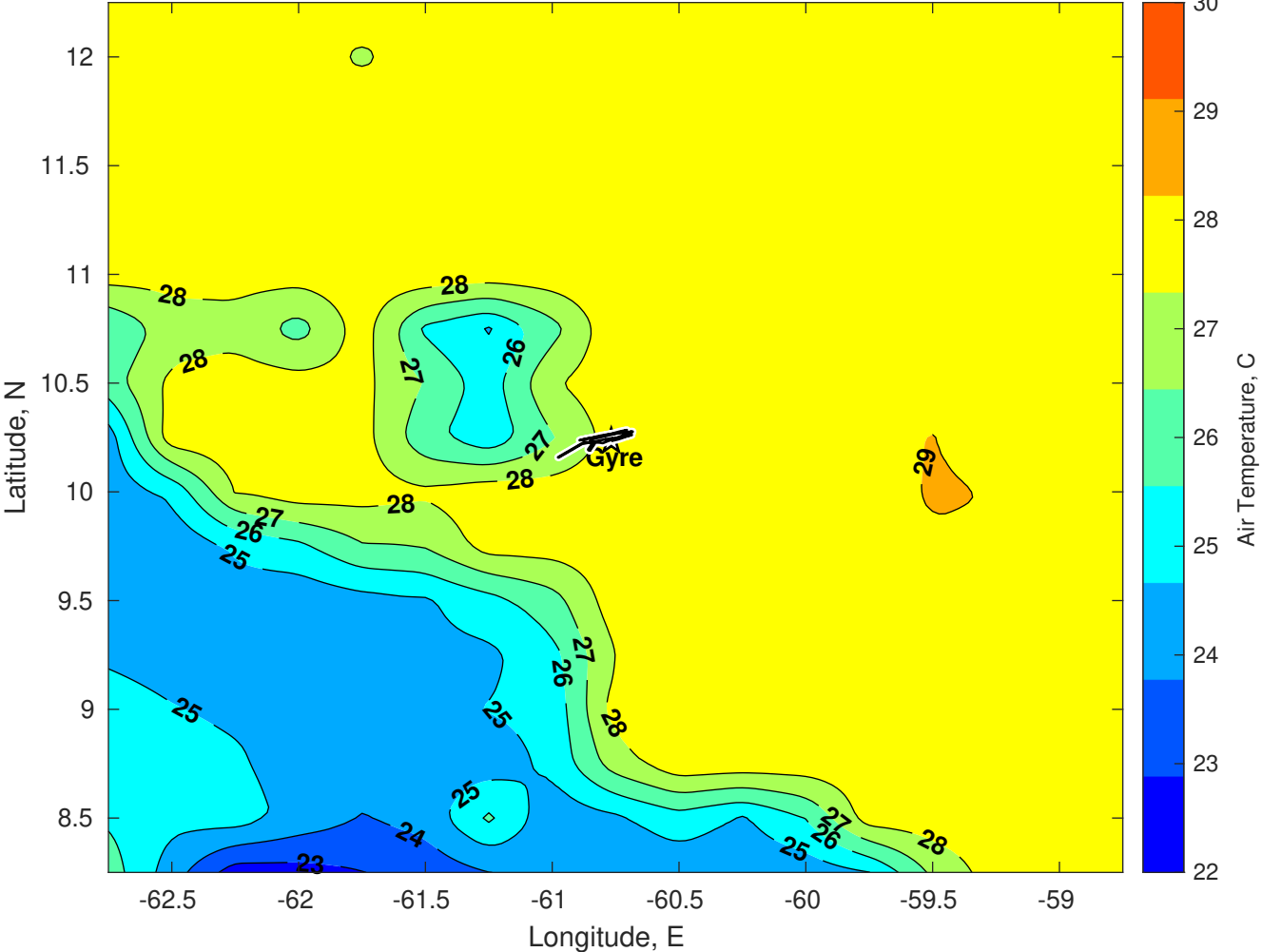
Air Temperature (C) for Gyre at 11-Nov-2025
