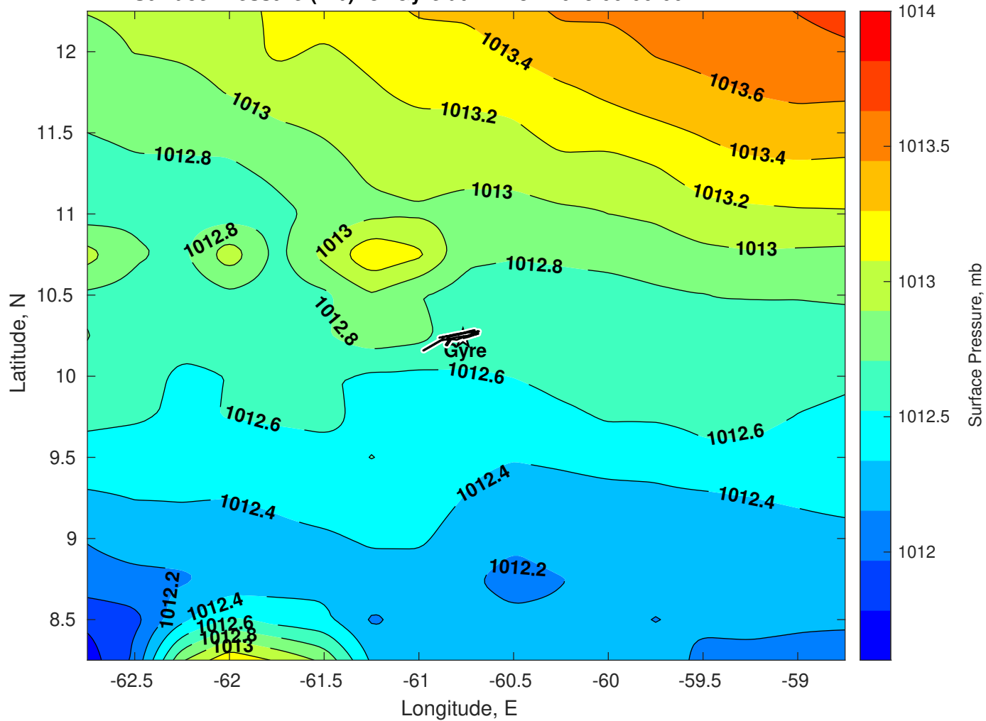
Surface Pressure (mb) for Gyre at 12-Nov-2025 00:00:00
