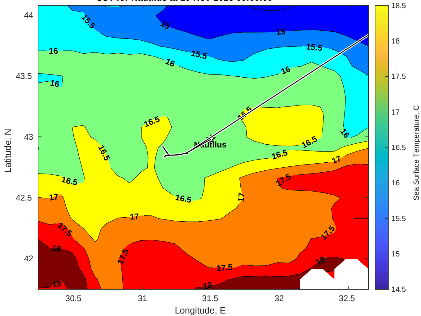
SST for Nautilus at 10-Nov-2025 00:00:00
