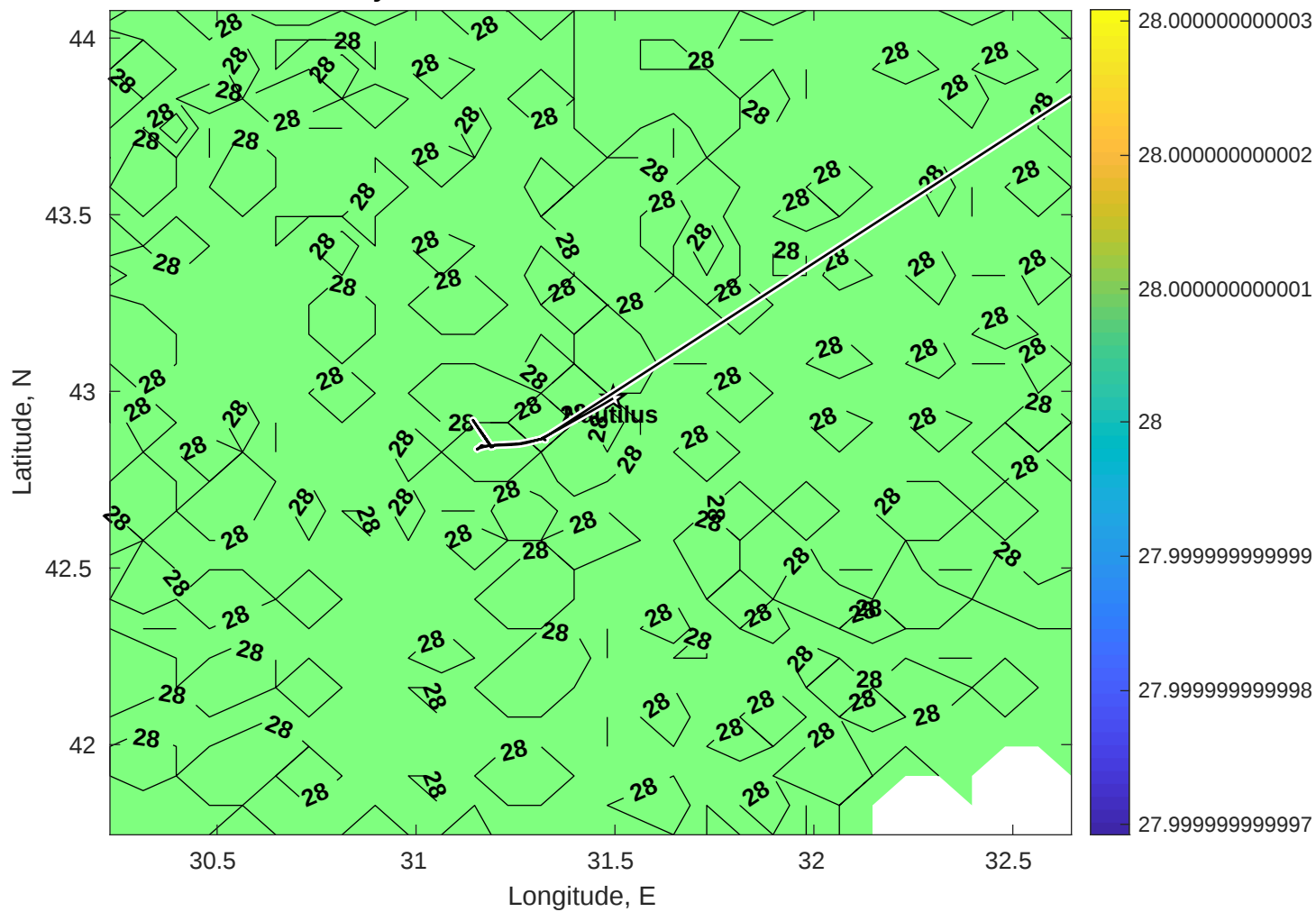
Surface Salinity for Nautilus at 10-Nov-2025 00:00:00
