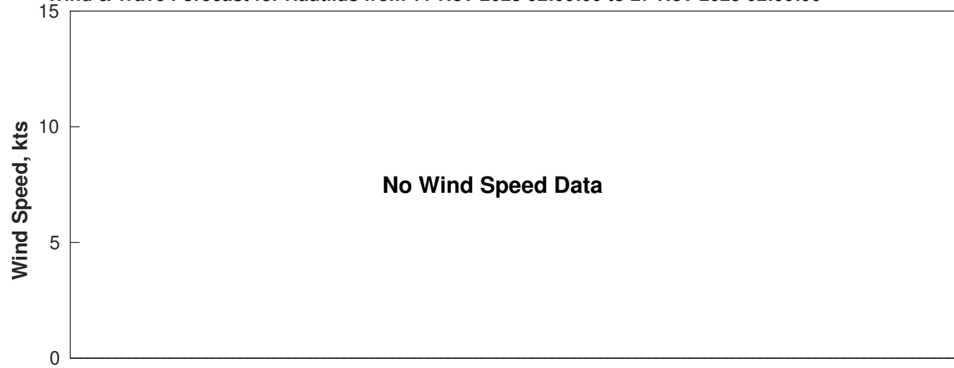
Wind & Wave Forecast for Nautilus from 11-Nov-2025 02:00:00 to 27-Nov-2025 02:00:00
