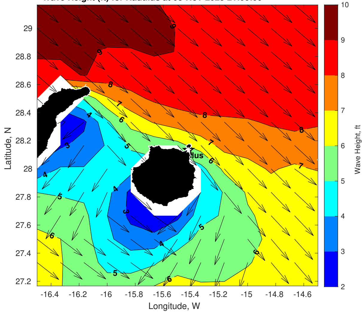
Wave Height (ft) for Nautilus at 08-Nov-2025 21:00:00
