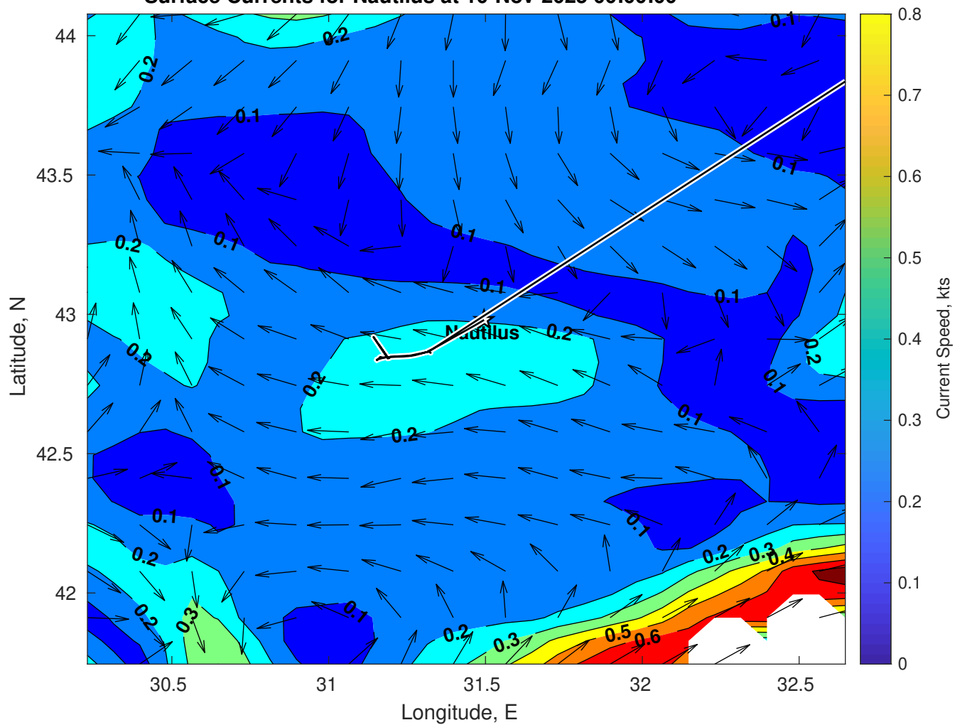
Surface Currents for Nautilus at 10-Nov-2025 00:00:00
