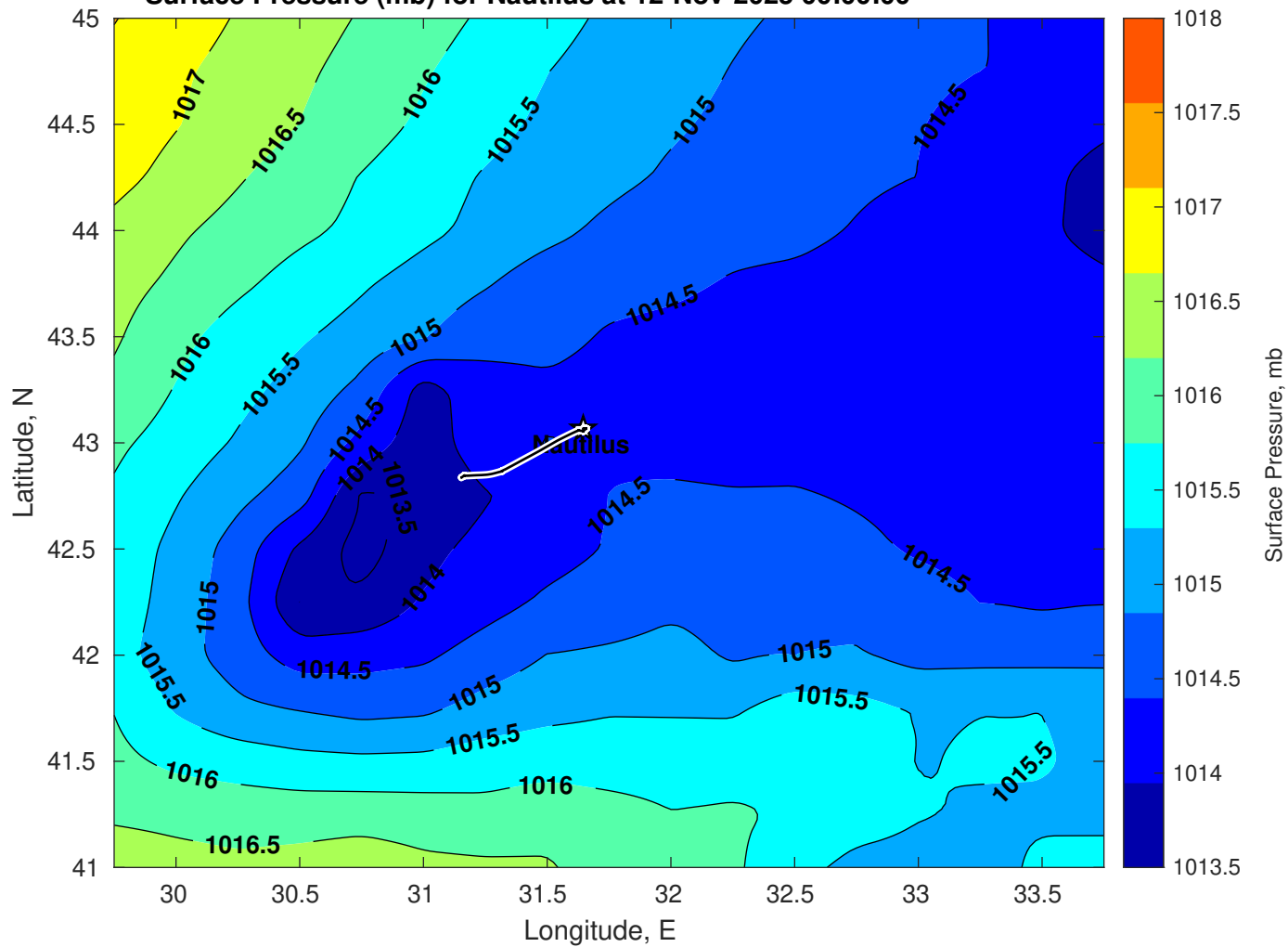
Surface Pressure (mb) for Nautilus at 12-Nov-2025 00:00:00
