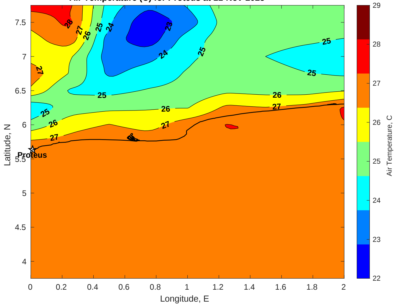
Air Temperature (C) for Proteus at 11-Nov-2025
