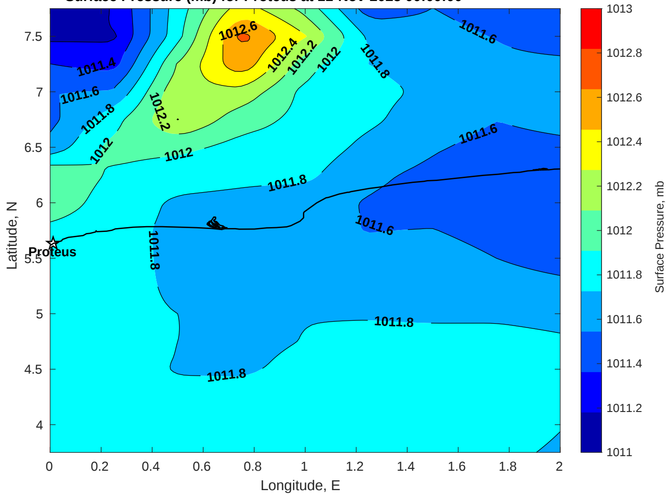
Surface Pressure (mb) for Proteus at 11-Nov-2025 00:00:00
