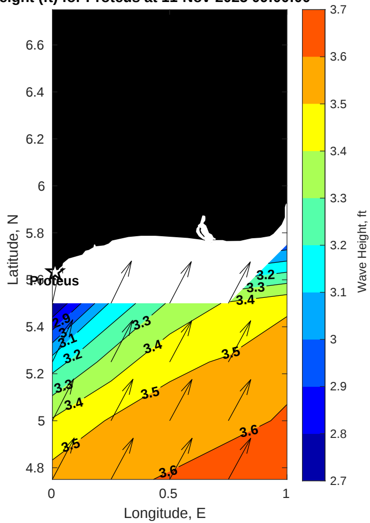
Wave Height (ft) for Proteus at 11-Nov-2025 09:00:00
