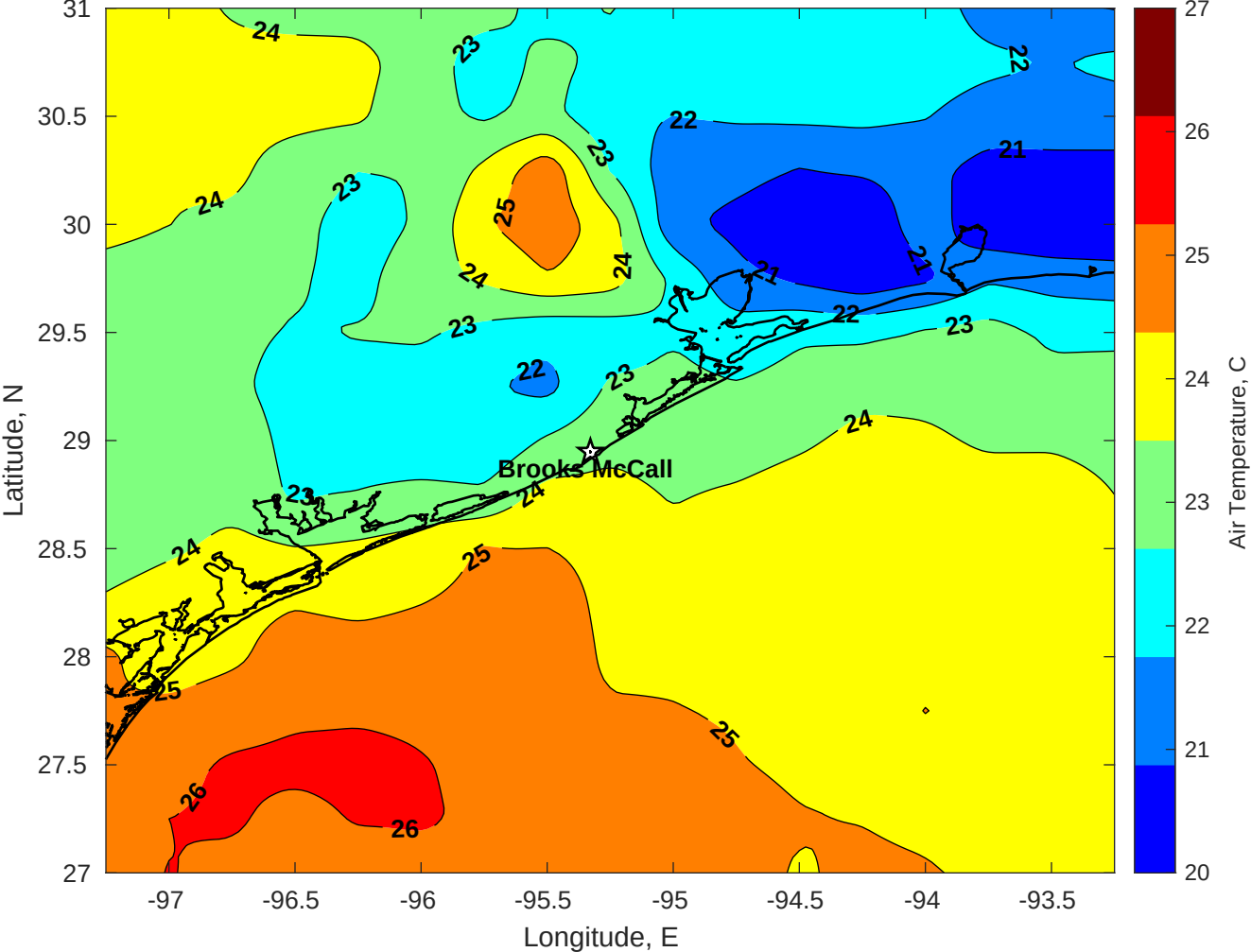
Air Temperature (C) for Brooks McCall at 12-Nov-2025
