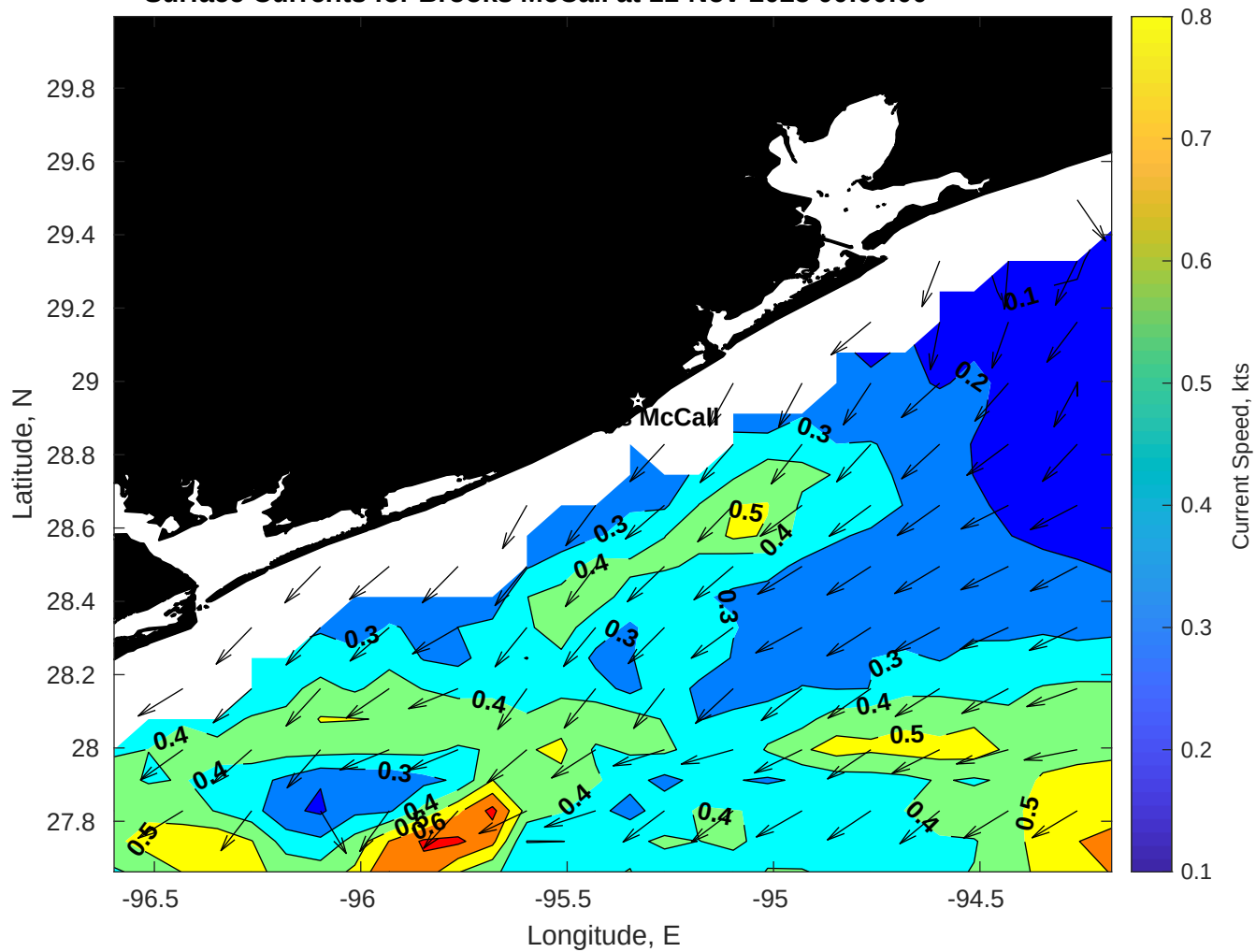
Surface Currents for Brooks McCall at 11-Nov-2025 00:00:00
