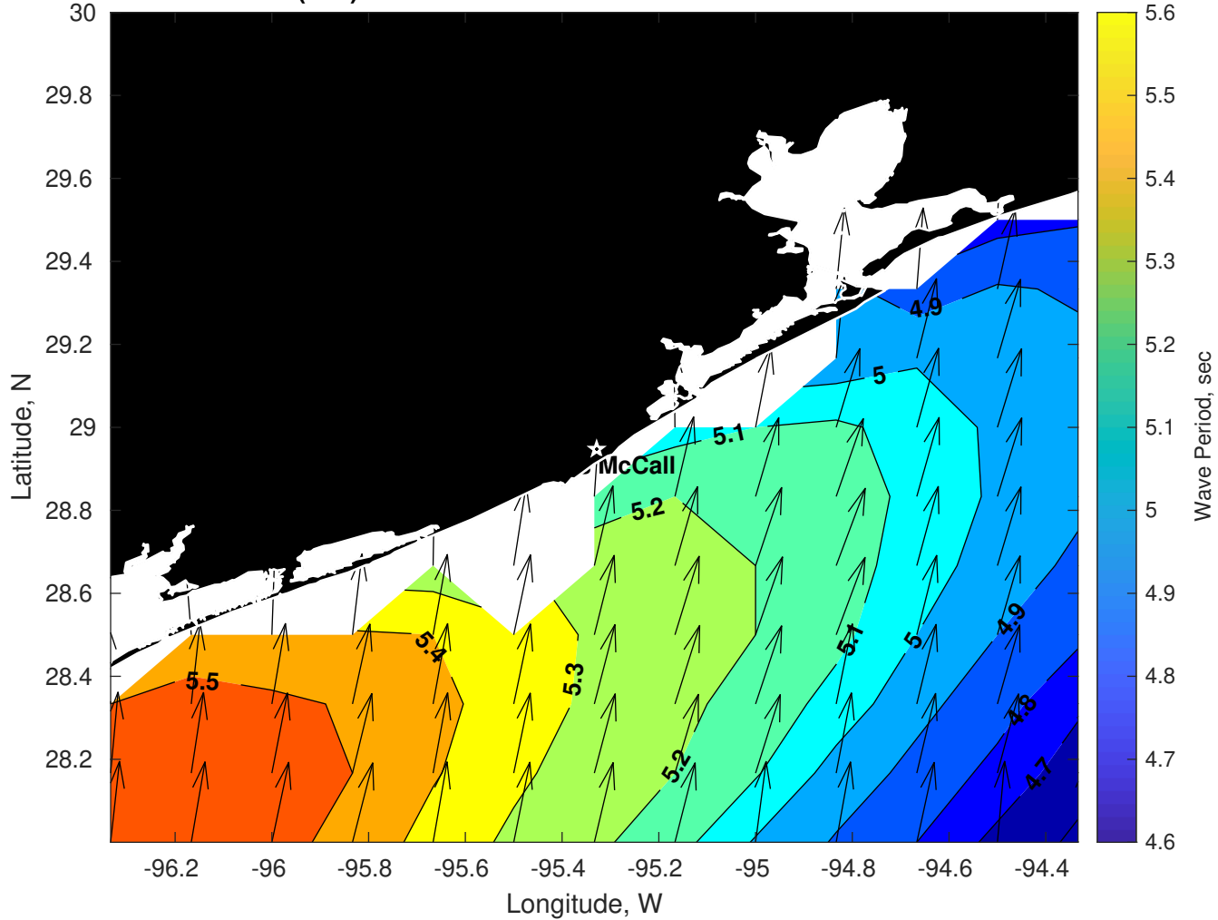
Wave Period (sec) for Brooks McCall at 12-Nov-2025 09:00:00
