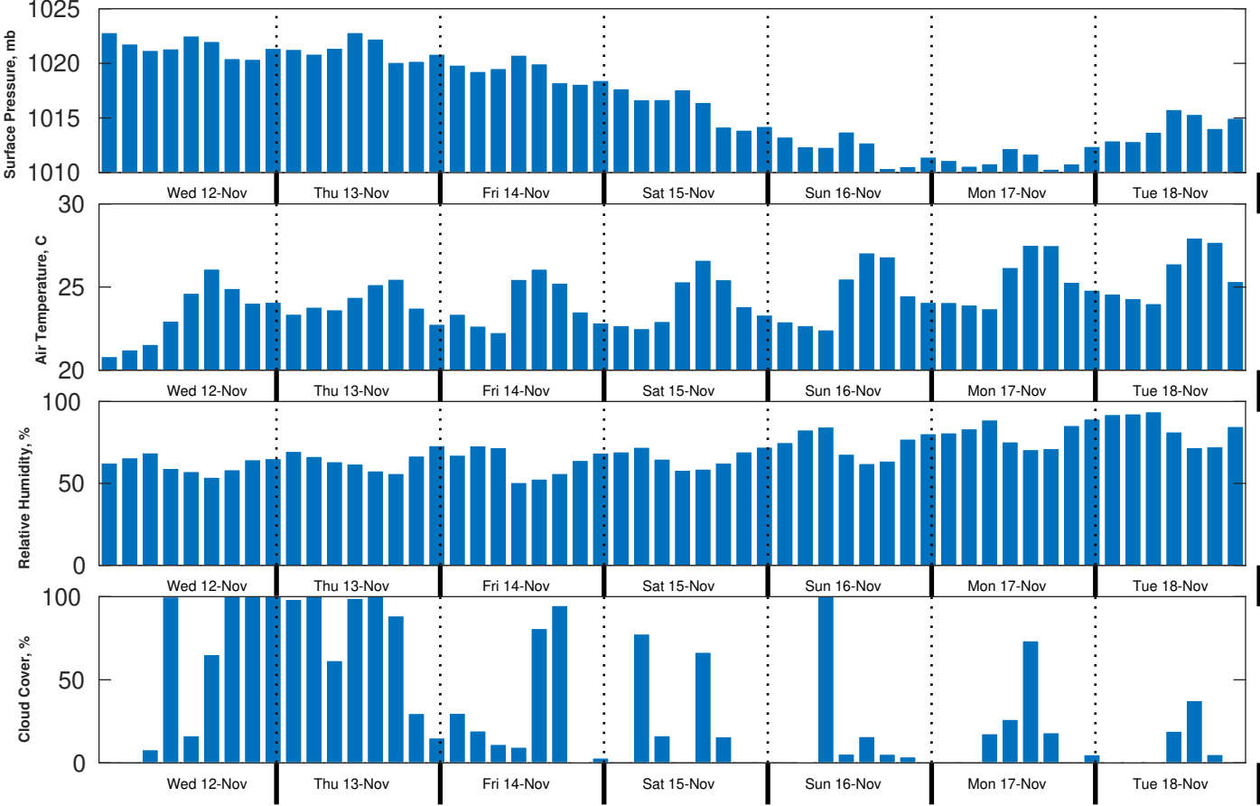
Met Forecast for Brooks McCall from 12-Nov-2025 00:00:00 to 19-Nov-2025 00:00:00
