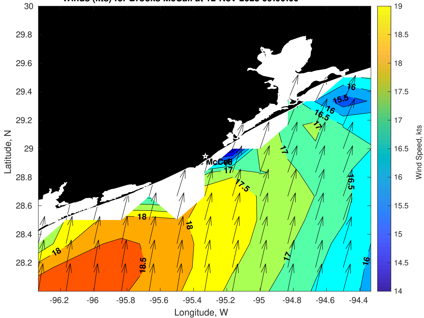
Winds (kts) for Brooks McCall at 12-Nov-2025 09:00:00
