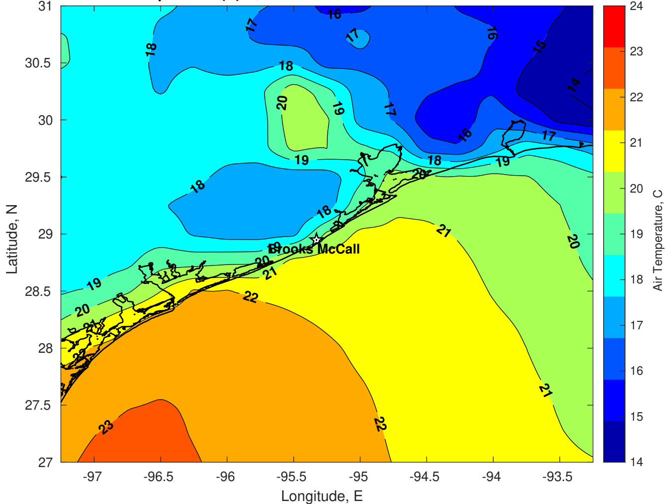
Air Temperature (C) for Brooks McCall at 12-Nov-2025
