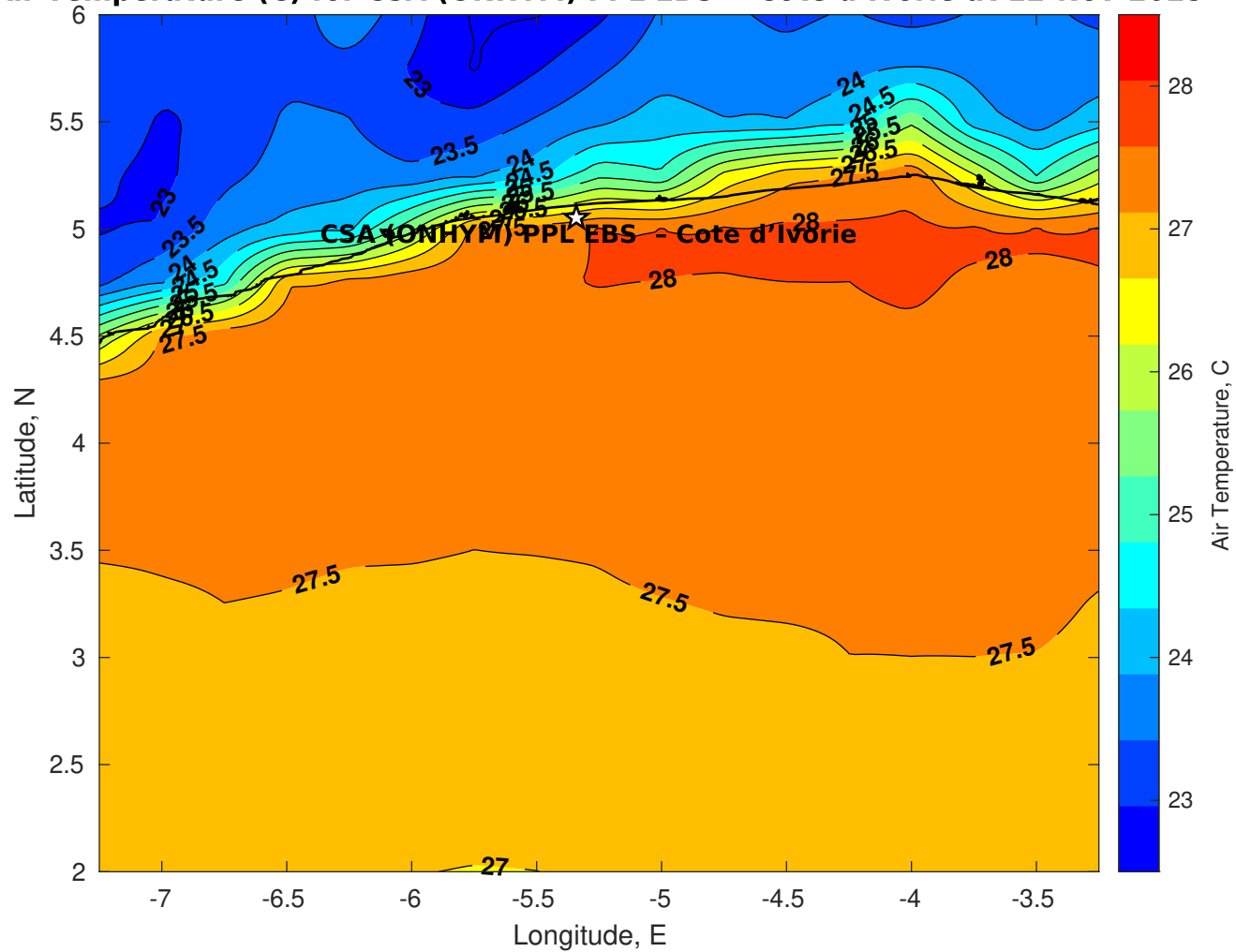
Air Temperature (C) for CSA (ONHYM) PPL EBS - Cote d'Ivoire at 12-Nov-2025
