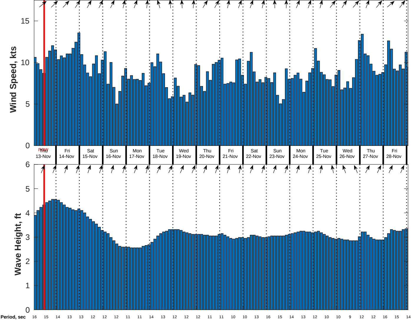
Wind & Wave Forecast for CSA (ONHYM) PPL EBS - Cote d'Ivoire from 12-Nov-2025 01:00:00 to 28-Nov-2025 01:00:00
