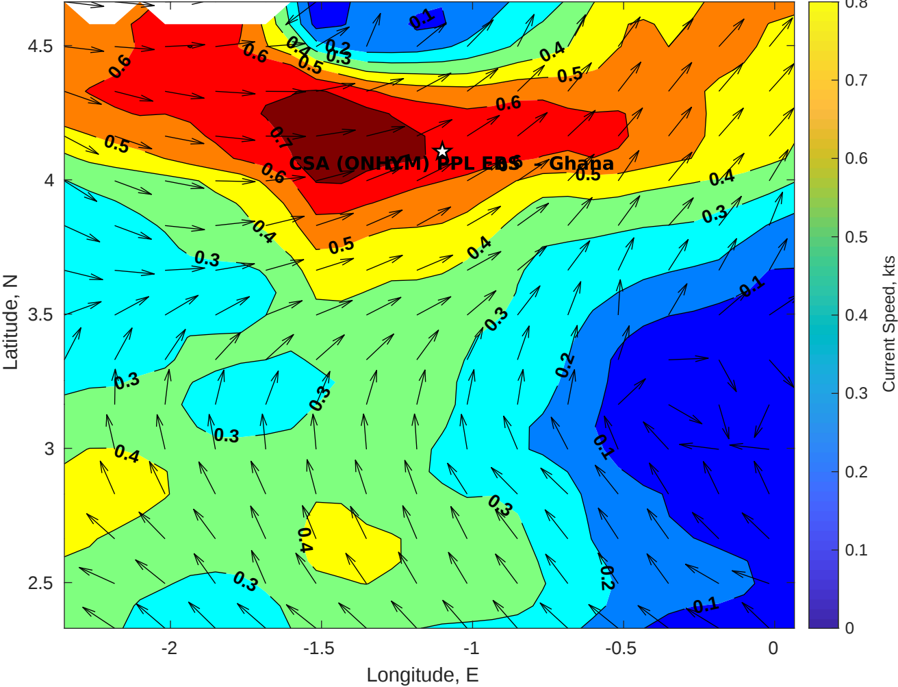
Surface Currents for CSA (ONHYM) PPL EBS - Ghana at 11-Nov-2025 00:00:00
