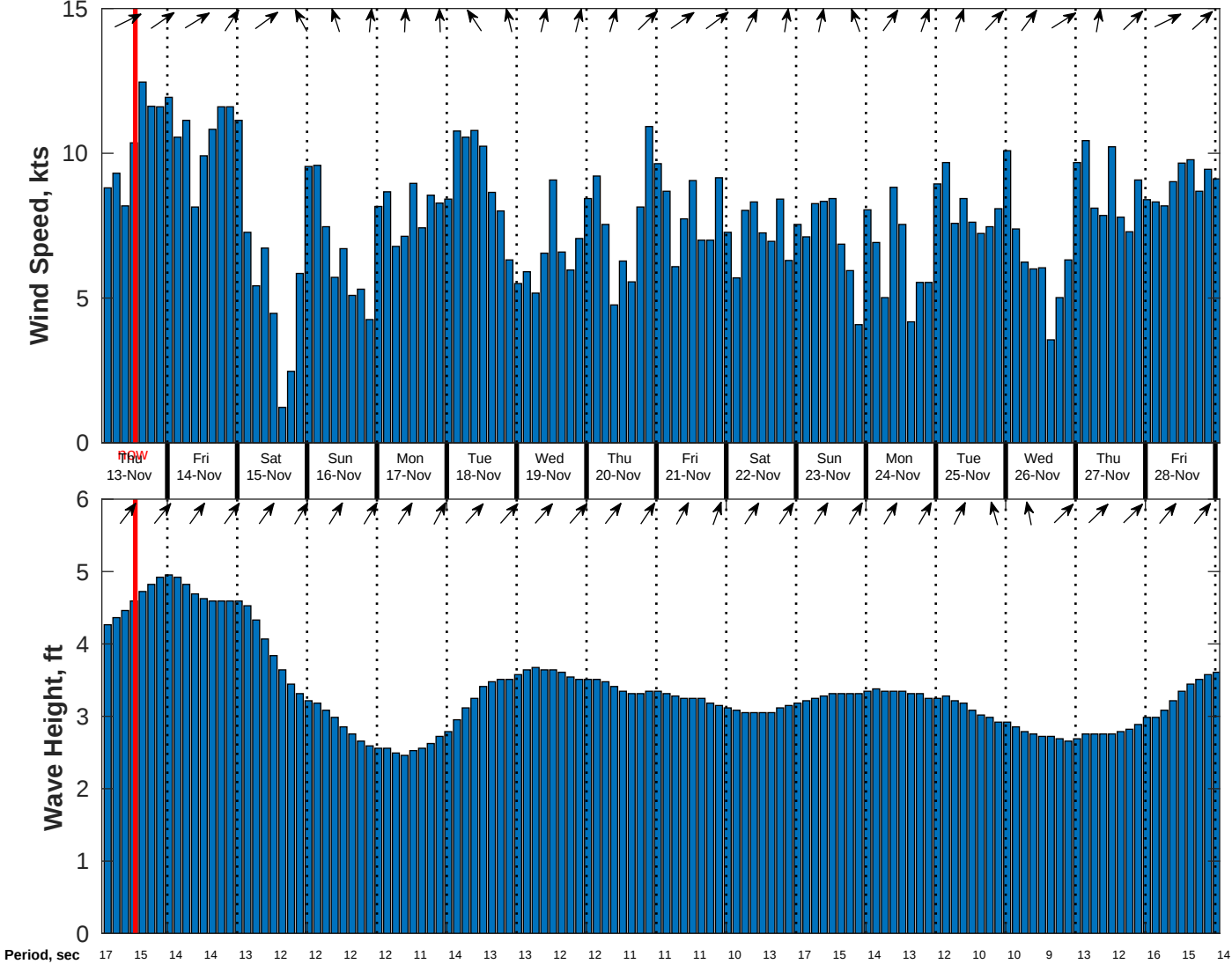
Wind & Wave Forecast for CSA (ONHYM) PPL EBS - Ghana from 12-Nov-2025 02:00:00 to 28-Nov-2025 02:00:00
