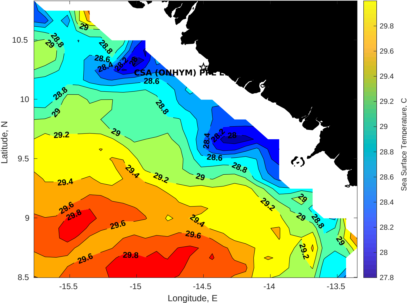
SST for CSA (ONHYM) PPL EBS - Guinea at 11-Nov-2025 00:00:00
