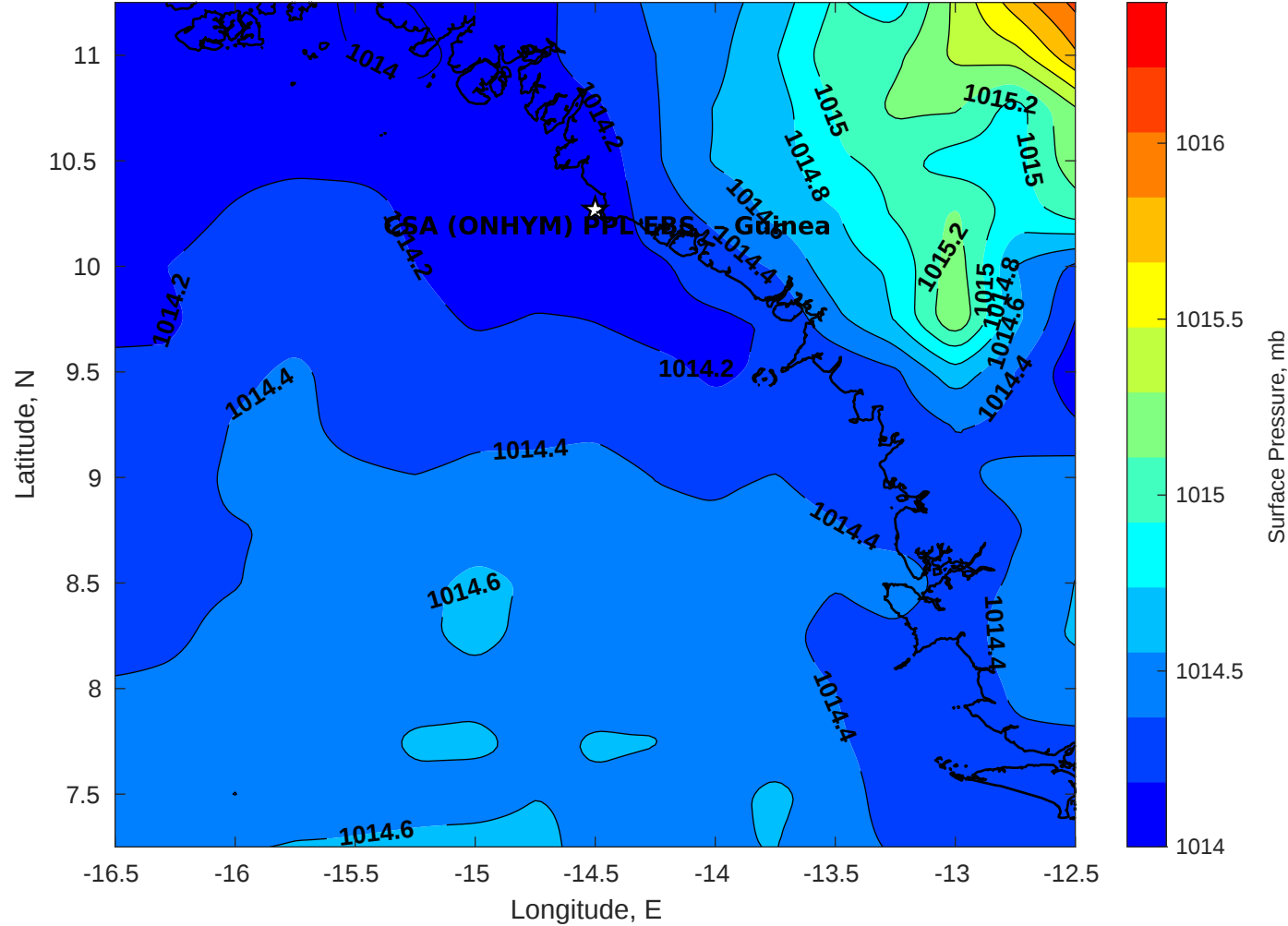
Surface Pressure (mb) for CSA (ONHYM) PPL EBS - Guinea at 14-Nov-2025 00:00:00
