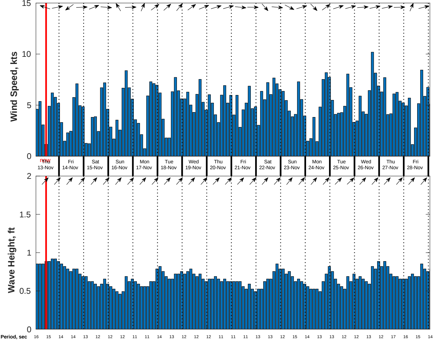
Wind & Wave Forecast for CSA (ONHYM) PPL EBS - Guinea from 12-Nov-2025 01:00:00 to 28-Nov-2025 01:00:00
