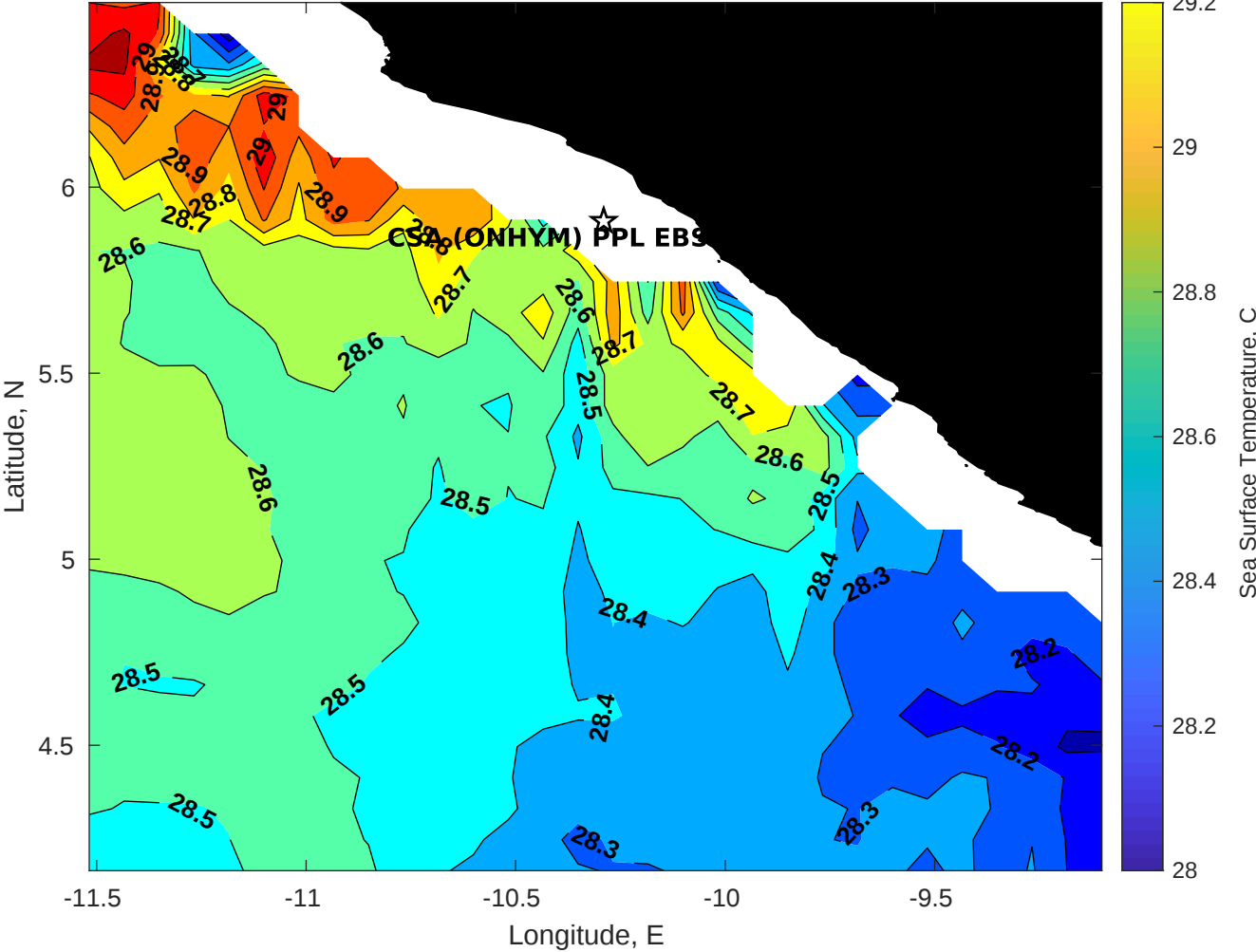
SST for CSA (ONHYM) PPL EBS - Liberia at 11-Nov-2025 00:00:00
