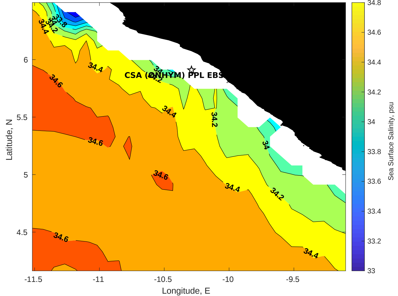
Surface Salinity for CSA (ONHYM) PPL EBS - Liberia at 11-Nov-2025 00:00:00
