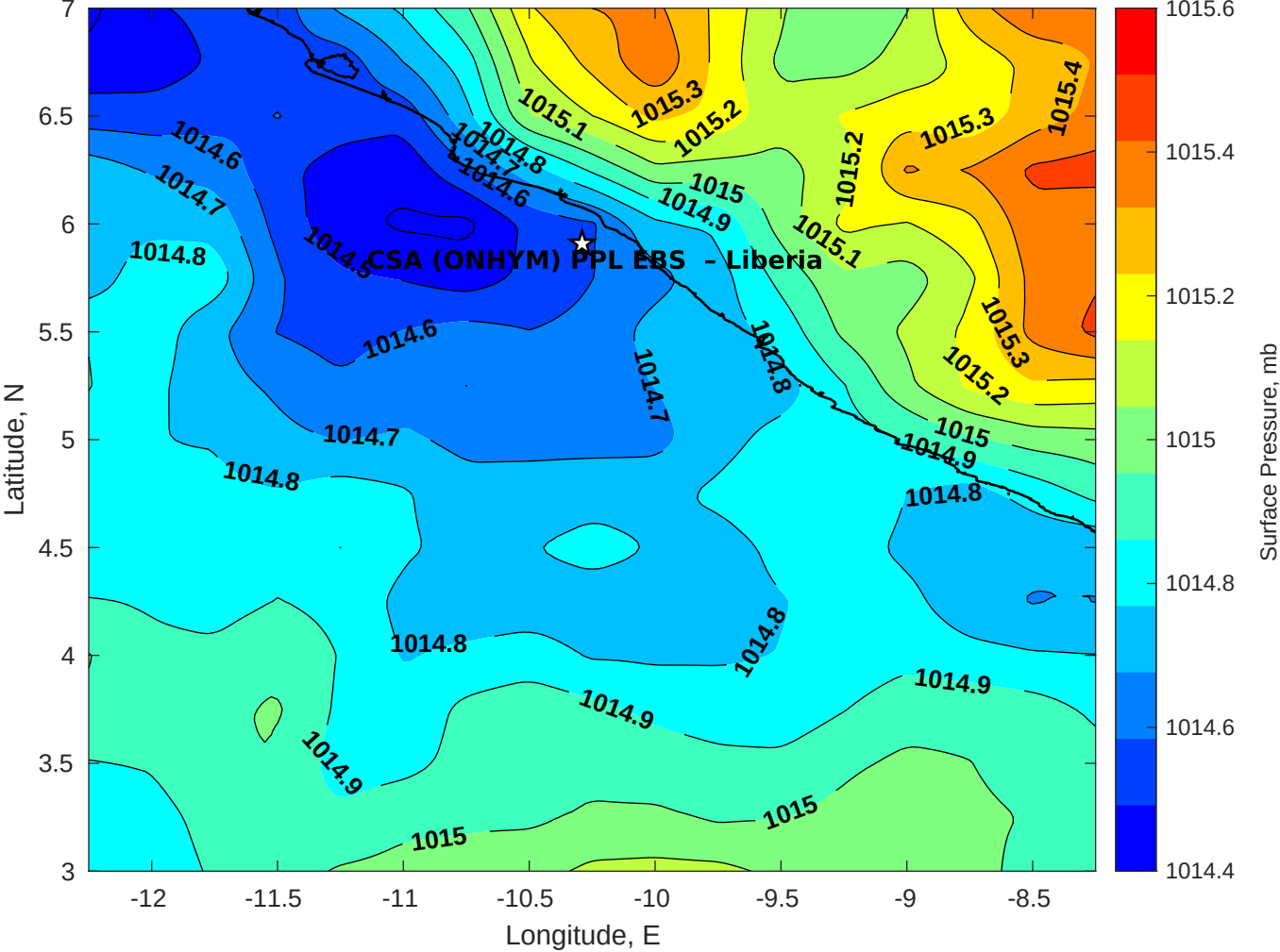
Surface Pressure (mb) for CSA (ONHYM) PPL EBS - Liberia at 14-Nov-2025 00:00:00
