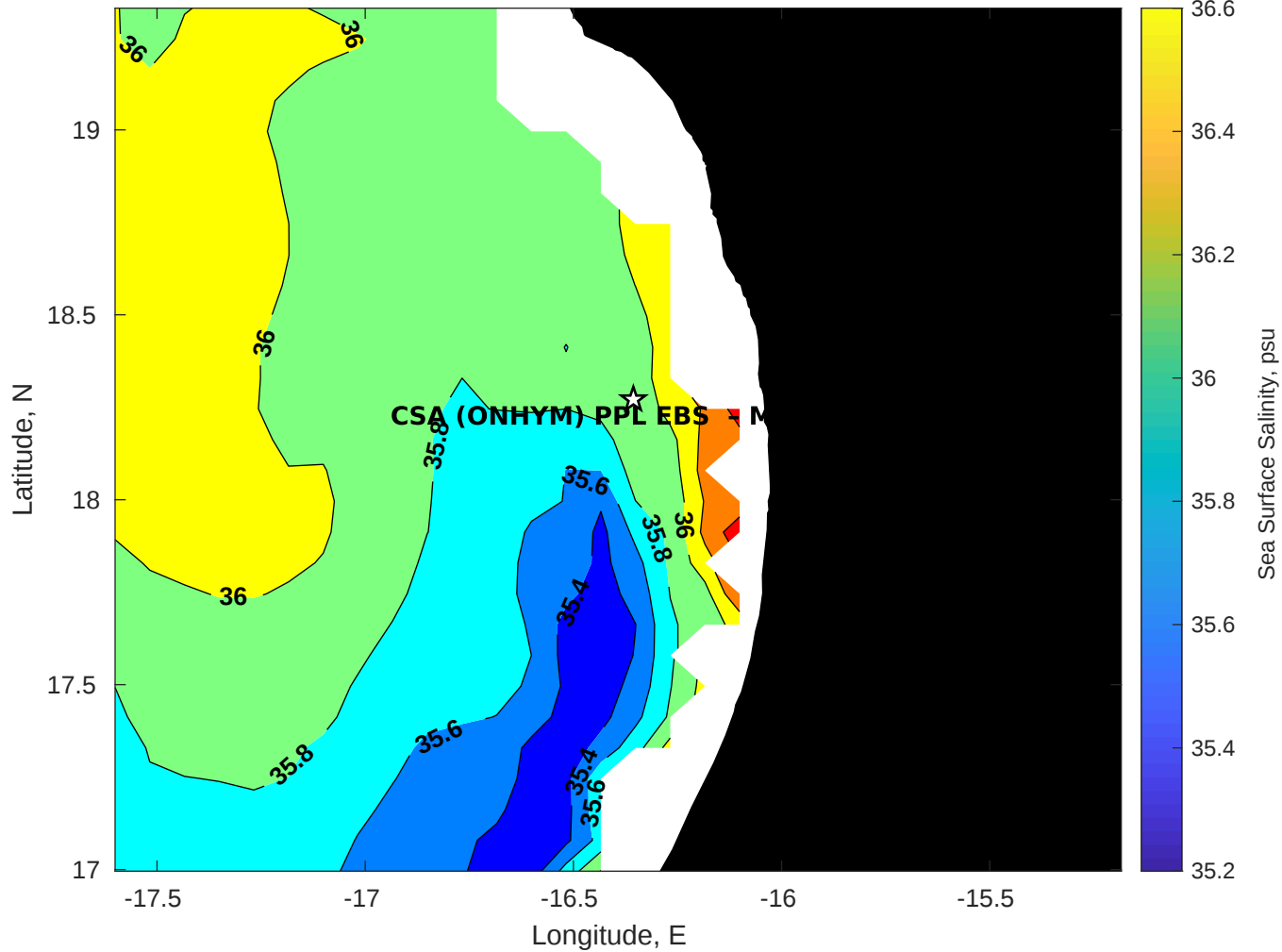
Surface Salinity for CSA (ONHYM) PPL EBS - Mauritania at 11-Nov-2025 00:00:00
