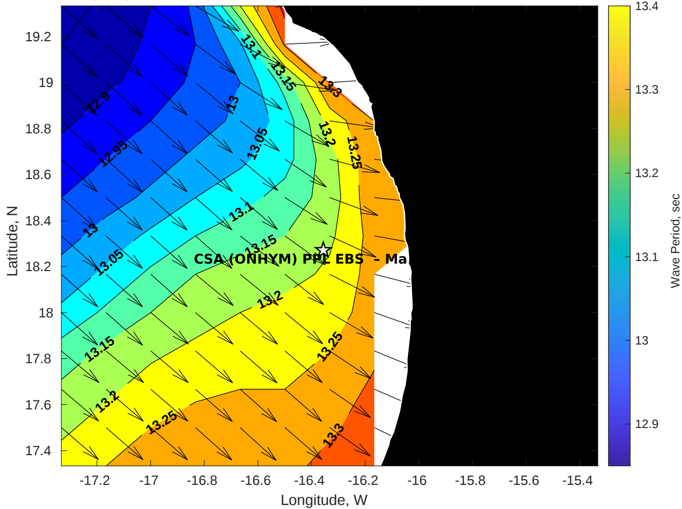
Wave Period (sec) for CSA (ONHYM) PPL EBS - Mauritania at 12-Nov-2025 09:00:00
